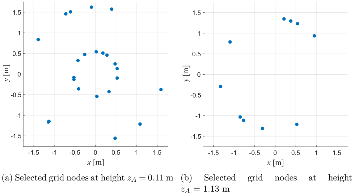
Figure 5.19: NB-R1 selected nodes on grid for some horizontal sections in xy -plane for grid value z_A along z
