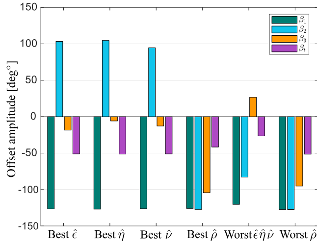
Figure 4.15: Offset amplitudes of best and worst design for indices \hat{e} , \hat{\eta} , \hat{\nu} and \hat{\rho} during the candidate selection phase obtained with the center of mass task
