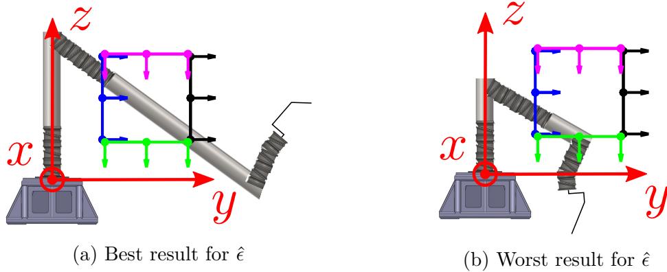
Figure 4.16: Representation of the design with the best and worst \hat{e} together with the four trajectories used during the optimization process, employing the center of mass task. The design parameter values are in the first line of Table 4.9.
