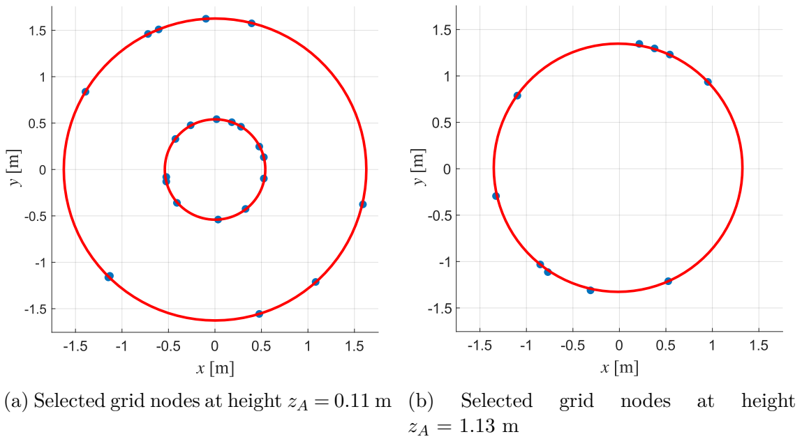
Figure 5.20: Reconstructed circumferences with center (x_c, y_c) and radius R_1 and R_2 starting from the NB-R1 selected nodes on grid for some horizontal sections in xy -plane for grid value z_A along z
