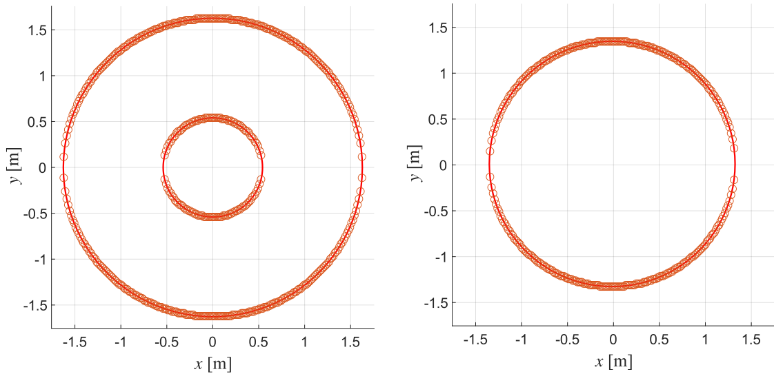
(a) Selected grid nodes at height z_C = 0.11 m (b) Selected grid nodes at height z_C = 1.13 m
