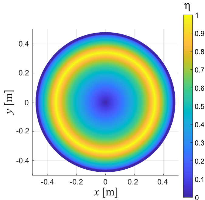
Figure 2.15: Dexterity \eta shown on NB-module workspace for r = 1 m and \alpha = \pi/12 rad = 15^\circ
