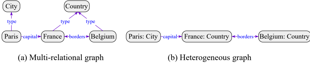
Figure 3.1: Illustrations of (a) multi-relational graph and (b) heterogeneous graph.
