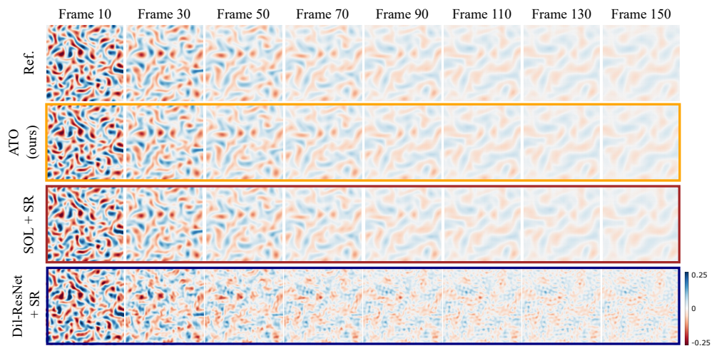
Figure 4.20: Example frames of a test case for different models for the decaying turbulence scenario. The vorticity fields are shown.
