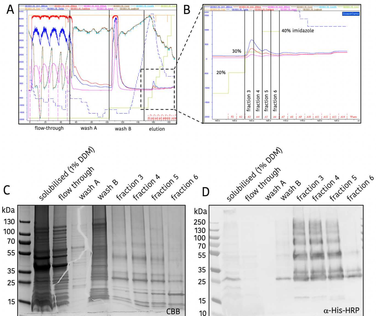
Figure 34. Affinity chromatography of Lgt-His purification. A) Analysis of flow, B) zoomed region where Lgt is eluted. C) Coomassie Brilliant Blue gel and D) \alpha -His-HRP Western-blot of samples, lanes relate to fractions noted in A).
