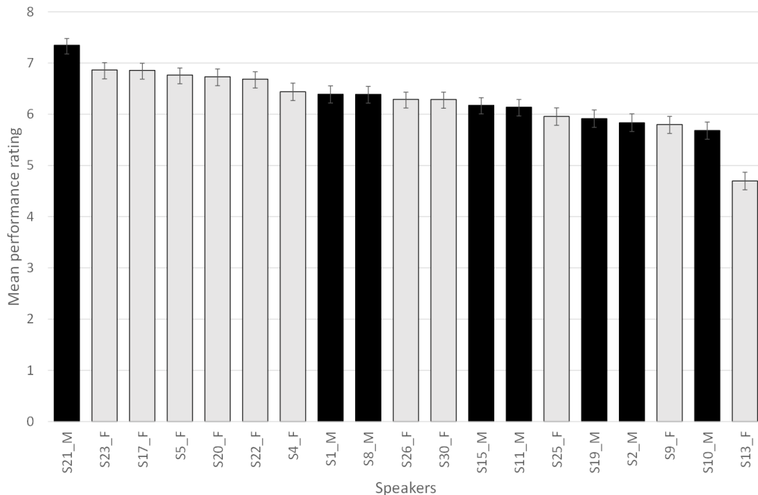
FIGURE II.3.1: Mean performance ratings for each speaker in decreasing order. Performance rating for male and female speakers are respectively displayed in black and grey. Error bars represent the 95% confidence interval
