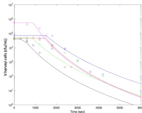
Figure 3: Kinetic inactivation curves obtained for the determination of the best fitting kinetic law : model N°3, (—) for I = 10 \text{ W} \cdot \text{m}^{-2} and C_0 = 10^5 \text{ cfu} \cdot \text{mL}^{-1} , (—) for I = 20 \text{ W} \cdot \text{m}^{-2} and C_0 = 10^5 \text{ cfu} \cdot \text{mL}^{-1} , (—) for I = 35 \text{ W} \cdot \text{m}^{-2} and C_0 = 10^5 \text{ cfu} \cdot \text{mL}^{-1} , (—) for I = 45 \text{ W} \cdot \text{m}^{-2} and C_0 = 10^5 \text{ cfu} \cdot \text{mL}^{-1} , and (—) for I = 35 \text{ W} \cdot \text{m}^{-2} and C_0 = 10^6 \text{ cfu} \cdot \text{mL}^{-1} ,
