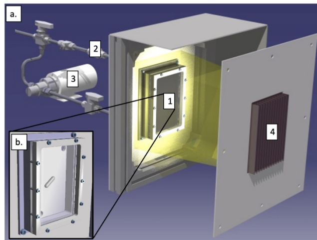
Figure 1: Presentation of the apparatus: pilot (a) composed of the photoreactor (1), the recirculating loop (2) with the centrifugal pump (3) and the UV LED panel (4). The figure (b) shows a closed view of the photoreactor.
