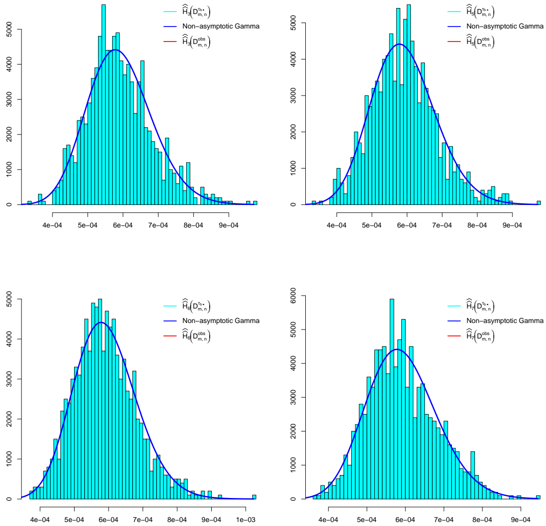
Figure 3.8: Superposition of histograms of \left\{ \widehat{\mathcal{H}}_j^2(D_{m,n}^{\tau_{b\bullet}}) \right\}_{1 \leq b \leq B_{\text{perm}}} (B_{\text{perm}} = 10^3) and Gamma distribution densities \Gamma(\tilde{a}_j, \tilde{b}_j) ( 1 \leq j \leq p ) relative to the calibration parameters k_v , A_2 and A_3 (Approach C).
