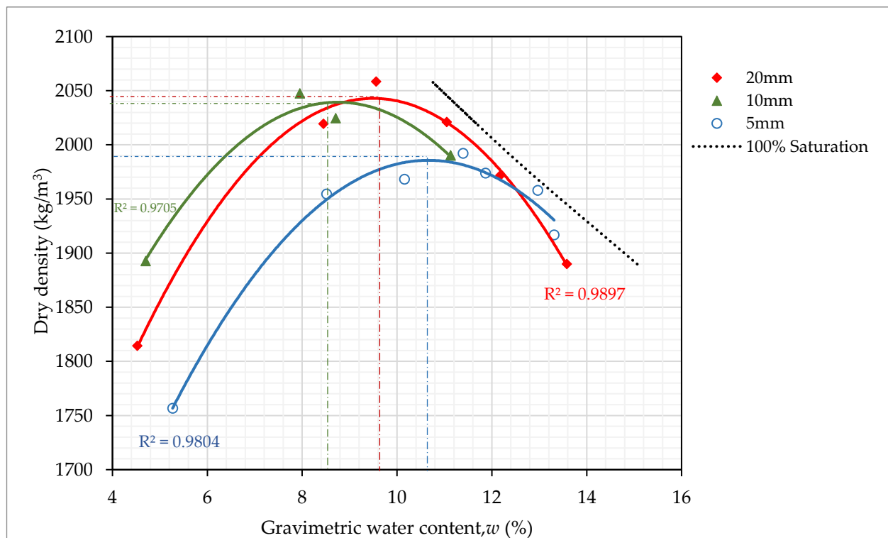
Figure 3.5: Modified Proctor test for soil with D_{\max} = 20 \text{ mm} , 10 \text{ mm} and 5 \text{ mm} .
