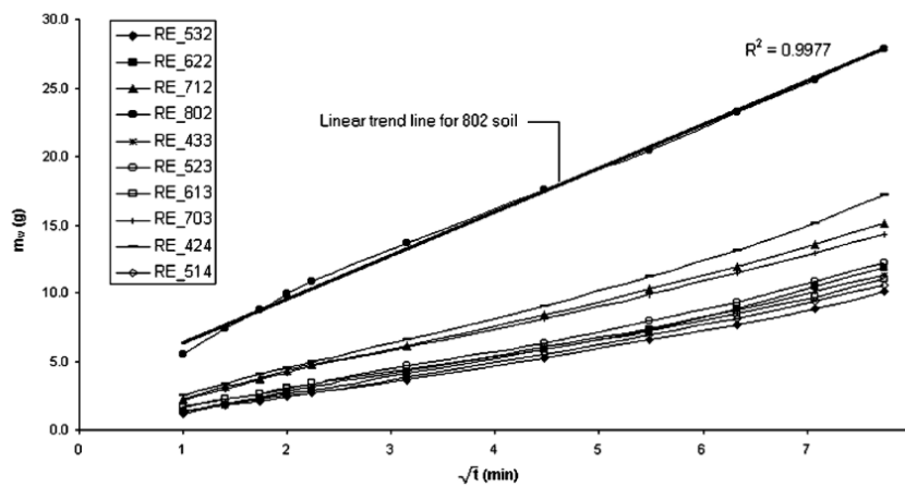
Figure 2.11: Relationship between the mass of absorbed water and the square root of elapsed time for different RE samples.
