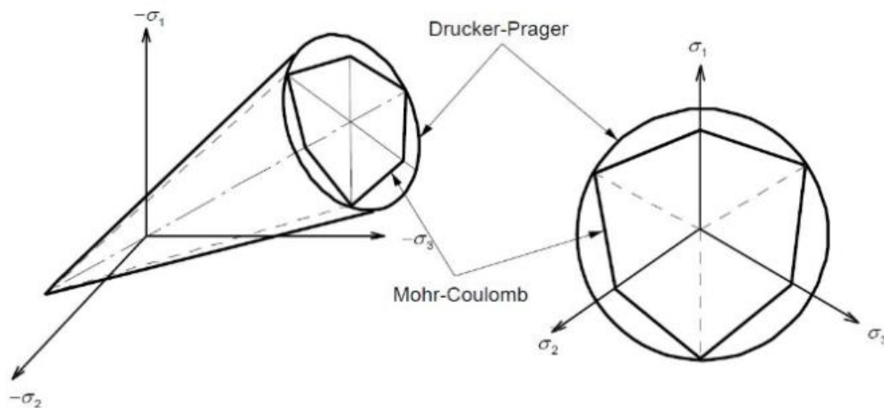
Figure 2.14: Mohr-Coulomb and the Drucker-Prager failure surface in (a) principal stress space and (b) in the octahedral plane.
