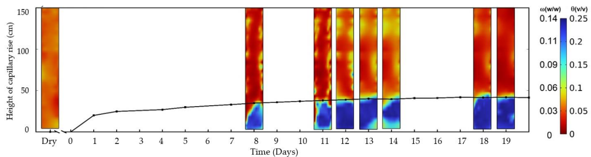
Figure 5.27: Water content (volumetric fraction) and (gravimetric fraction) tomograms obtained using induced polarization method [151].
