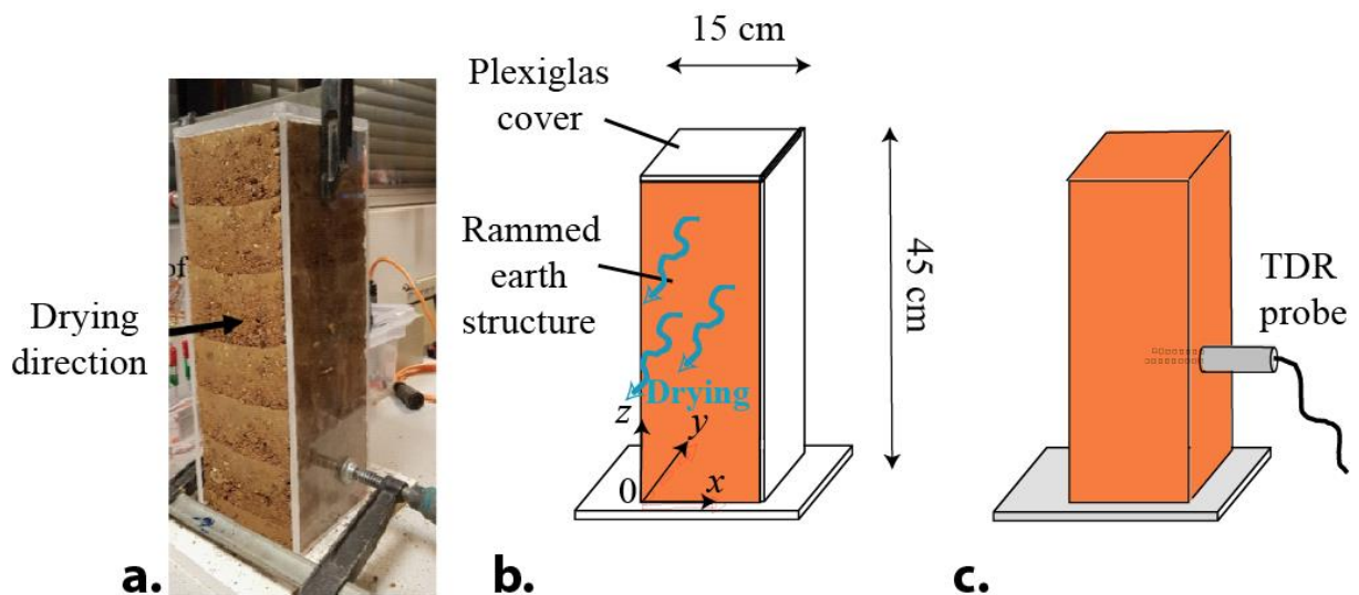
Figure 15. Rammed earth structural element. a. View of the earth structure S1 at manufacture with Plexiglas covering. We clearly see the six layers of rammed earth material. b. Sketch of the geometry for samples S1, S2, S3, with x , y , z axes. Drying is occurring from two lateral sides of the rammed earth element (the others being covered by Plexiglas layers). c. Sketch showing the position of the TDR sensor during the measurements for sample S1 (position y = 7.5 \text{ cm} , z = 20 \text{ cm} ). The TDR probe is used to get an independent estimate of the water content.
