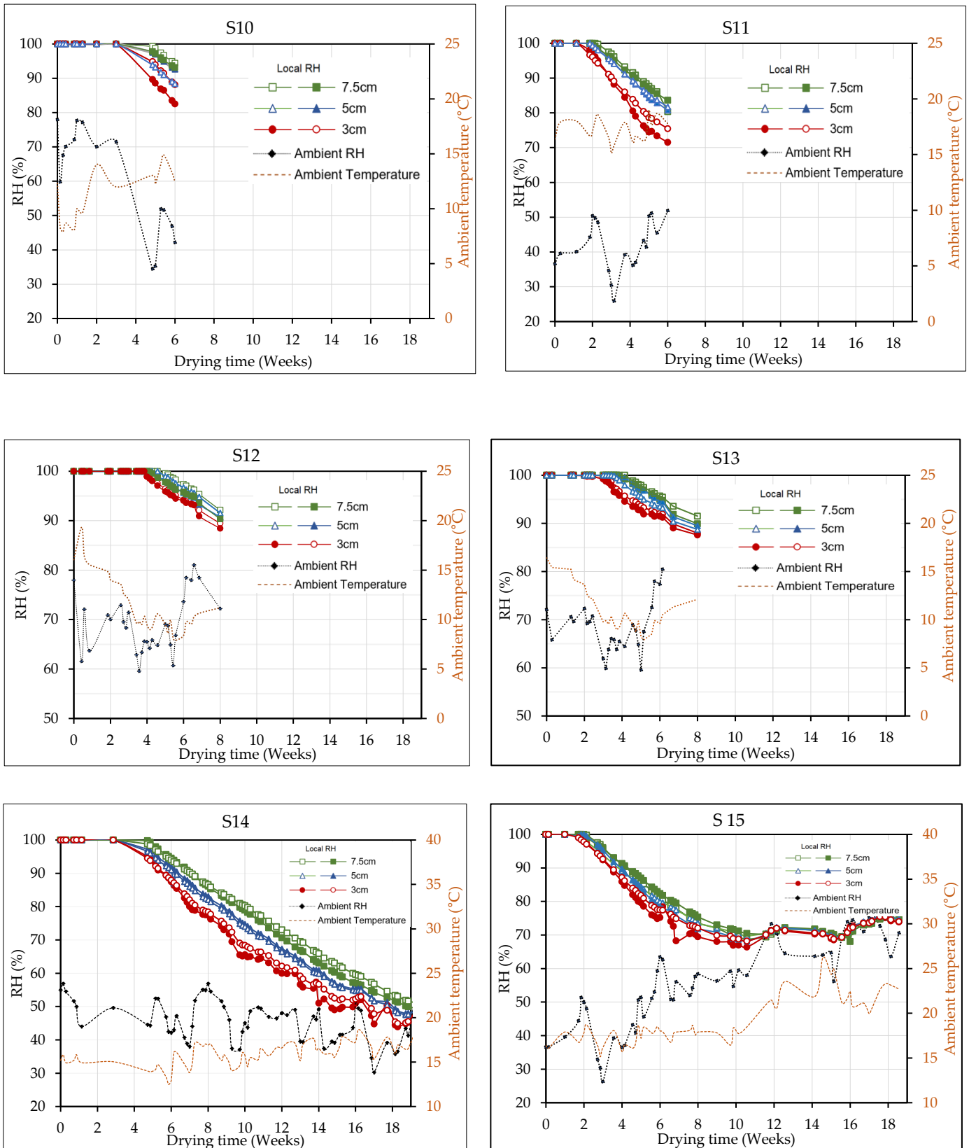
Figure 4.15: Evolution of RH with time for samples dried after 6, 8 and 19 weeks along with the variation of ambient RH and temperature (RH in samples measured by capacitive sensors at different depths: 3 cm, 5 cm and 7.5 cm) [133].
