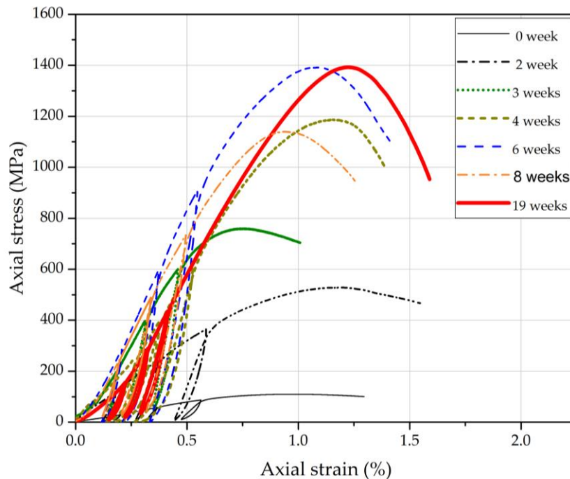
Figure 4.26: UCS with loading and unloading cycles of samples at different drying times [133].
