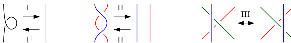
Figure 4.1: Reidemeister moves
