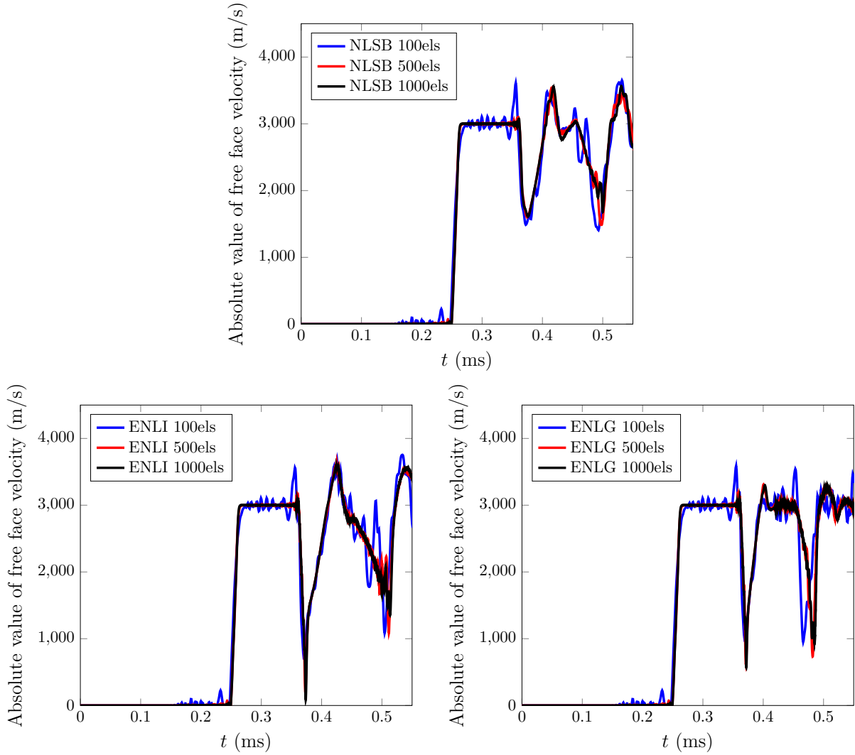
Figure 3.18 • NLSB (top), ENLI (left), and ENLG (right) damage models – Mesh convergence of the free-surface velocity response.
