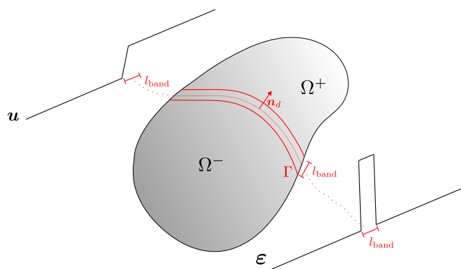
(b) Kinematics of a weak discontinuity
