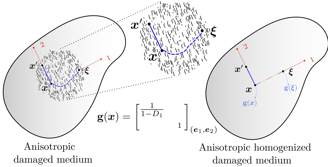
Figure 4.4 • Illustrative scheme of the Riemannian metric in an anisotropic damaged medium.
