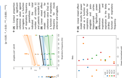
FIGURE 2: IEEG coherence with respiration depends on the respiratory situation
