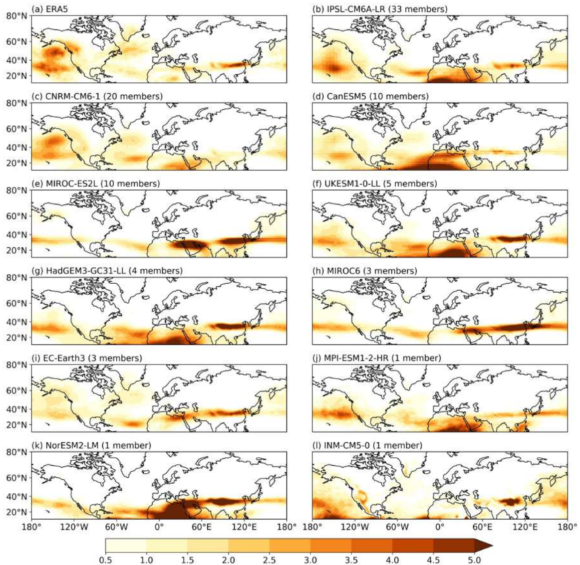
Figure 3.4 – Winter (DJF) climatology of MOG-CAT frequency ( \geq 0.5\% ) of vertical wind shear diagnostic at 200-250 hPa between 1981-2010 from (a) ERA5 reanalysis and (b-l) different CMIP6 climate models. Units are in %.
