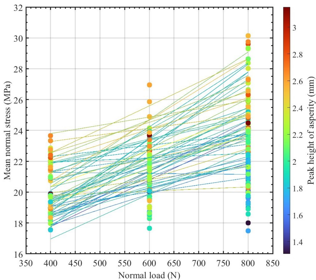
Figure 5.12: Mean normal stress as a function of the nominal normal load. The symbols are the measurements given by the pressure-sensitive film and are coded by the peak height of asperity. A best linear fit is presented when the asperity is detected by the pressure-sensitive film under all three normal loads, which is color-coded by the peak height of this asperity. It gives the linear relationship between mean normal stress on a local asperity with a specific peak height and the applied nominal normal load.
