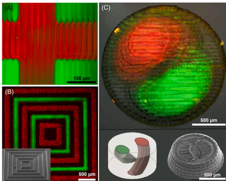
Fig. 8. Demonstration of multimaterial printing. (A) Successive printing of segments showing low cross contamination and alignment resolution, h = 50 \mu\text{m} . (B) Concentric squares printed from larger to smaller, h = 50 \mu\text{m} . (C) Double helicoidal structure, h = 500 \mu\text{m} . Lower left and right corners show a CAD image and a SEM image of the printed structure. (A-B-C) All made from PEGDA solutions (with 300-nm mCherry particles for red, 200-nm GFP particles for green, and no nanoparticles for grey).
