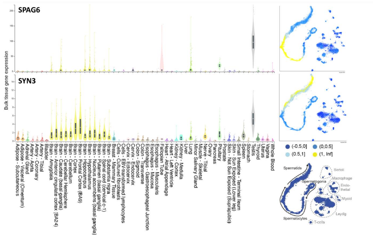
Figure 7.4 : Expression profiles of SPAG6 and SYN3 candidate genes in family 3 from Malakand phase 1
