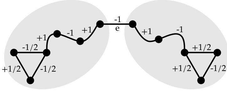
Figure 2.1: A way to change the weight of a non-static edge e \in E(G) \setminus S(G) without changing the vertex perimeters.
