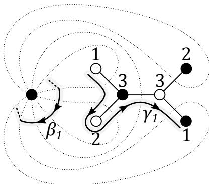
Figure 4.2: Construction of the curve \beta_i .
