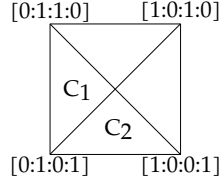
Figure 3.1: Projectivization of the cone H_{2,2}^+
