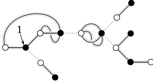
Figure 4.3: A degenerate graph with t = 5 components. The zero-length bridges are dotted. We have marked the black vertex number 1.
