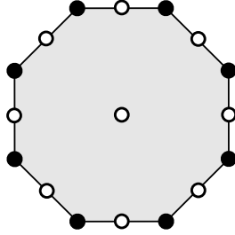
Figure 4.1: A surface of genus g = 2 from the hyperelliptic connected component \mathcal{H}^{hyp}(2) . The black points represent the singularity, while the white points represent 2g + 1 = 5 other fixed points of the “central symmetry” \sigma .
