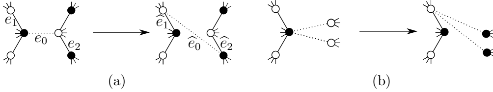
Figure 3.2: Flipping zero-weight edges.
