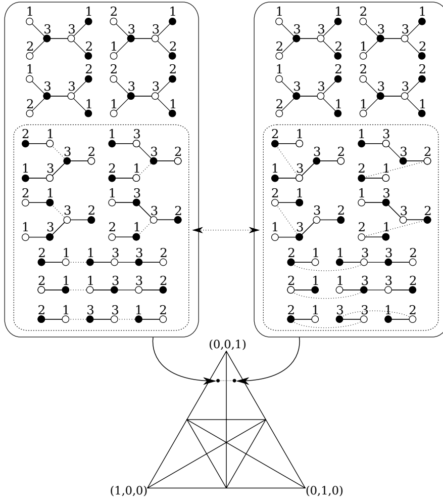
Figure 3.3: Illustration to the proof of Theorem 3.2 for g = 0 , where k = l = 3 , W = \{L_1 = L'_1, L_2 = L'_2, L_3 = L'_3\} , V = \{L_1 = L_2\} . At the bottom of the figure we see the projectivization of the three-dimensional cone H_{k,l}^+ \cap W = \{L_1 = L'_1, L_2 = L'_2, L_3 = L'_3, L_1 > 0, L_2 > 0, L_3 > 0\} . The cone is divided by 6 codimension 1 subspaces from \overline{W_{k,l}} into 12 “cells”. The number of trees positive at each point inside of each cell is the same (11 in this case). At the top of the figure are given the sets of positive trees corresponding to two particular points of the cone. Going from one of the points to the other, we must cross the subspace V . When we reach V from one side, certain trees cease to be positive — some of their edges become zero-weight (these edges are marked by dotted lines). In turn, when we continue to the other cell, certain trees become positive. The flipping procedure described in the proof provides a bijection between these sets of trees. In the figure, the corresponding trees are opposite to each other.
