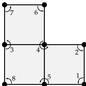
Figure 1.4: Identifying the opposite sides of this non-convex octagon, one obtains a surface of genus 2 tiled with 3 squares. All of the vertices of the squares are identified together into one conical singularity of angle 12 \cdot \frac{\pi}{2} = 6\pi . The numbered arrows represent the order in which the corners are visited when going around the singularity.
