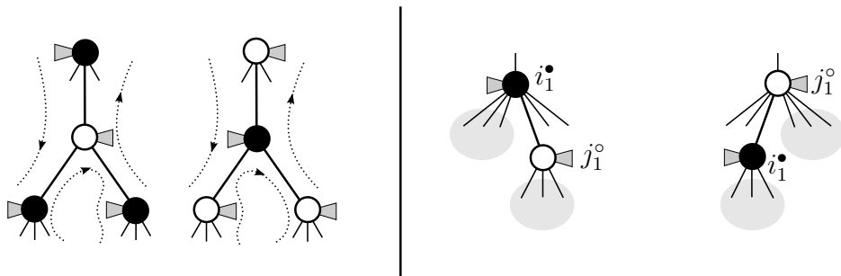
Figure 5.6: Proof of Lemma 5.14
