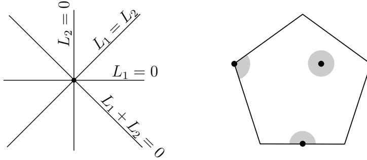
Figure 2.2: Left: polyhedral subdivision \mathcal{PS}_2 of \mathbb{R}^2 . Right: cones of feasible directions to a polygon in \mathbb{R}^2 at three points.
