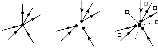
Figure 6.4: Left and center : exploding a vertex of G to construct G' . Right : local rule for constructing G'' (vertices are squares, edges are dashed).
