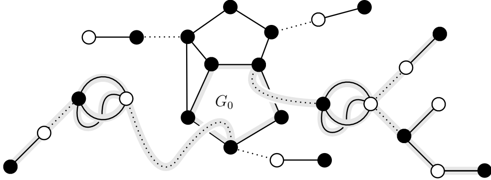
Figure 7.1: A degeneration of a ribbon graph G in \mathcal{RG}_{g,n}^{k,*} into 9 components. The zero-weight static bridges are dotted. The unique non-bipartite component G_0 has 4 faces of degrees 7, 5, 5, 3. Two “branches” are glued to the corners of one of the faces of degree 5. Their boundaries (in grey) form together a face of the initial graph G .
