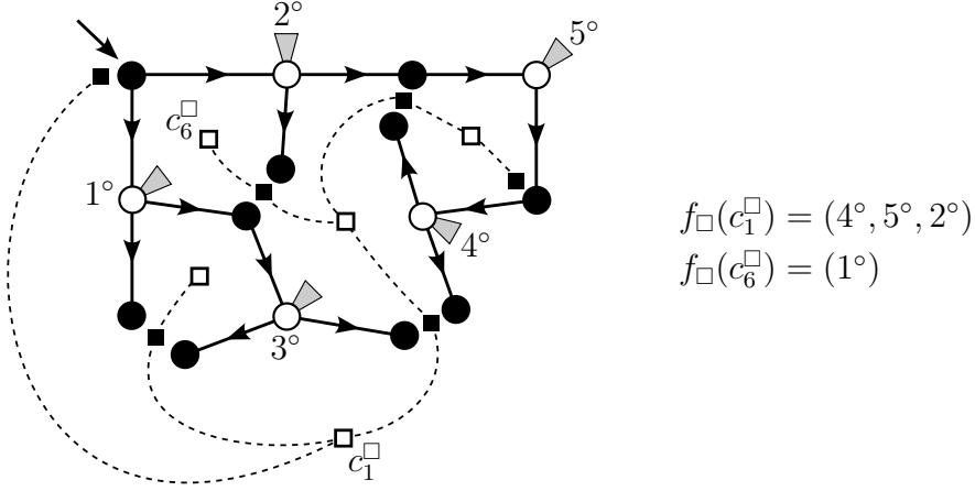
Figure 6.8: Definition of f_{\square} (decoration of the white corners of \bar{T} ).
