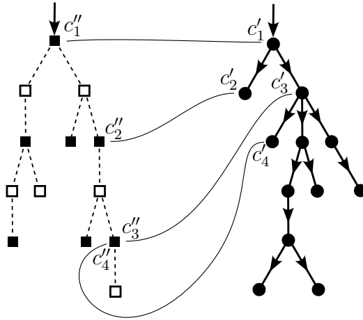
Figure 6.5: Gluing corners of G' and G'' to reconstruct G .
