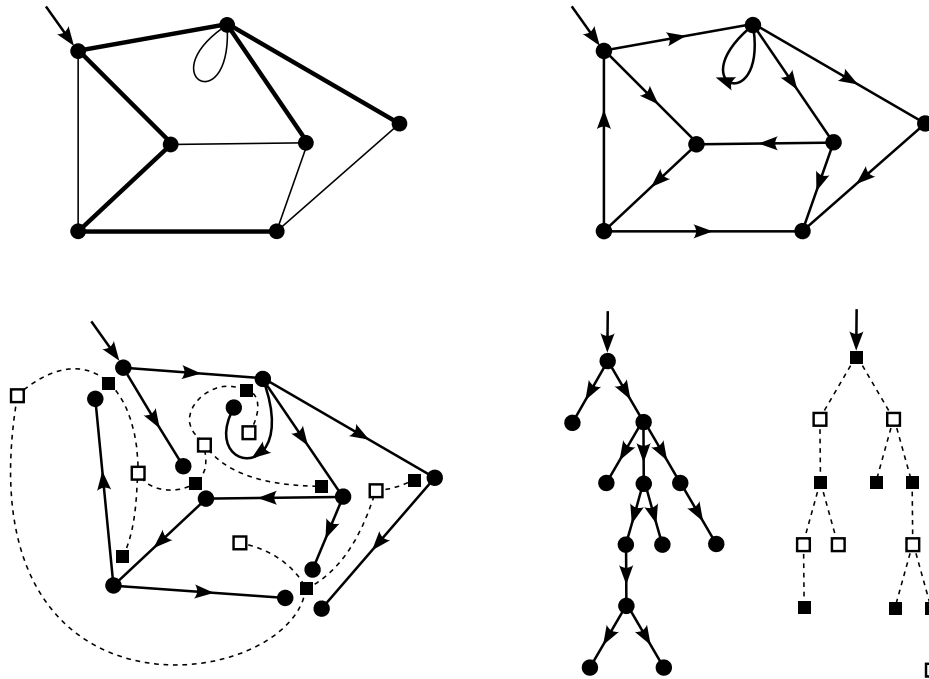
Figure 6.3: Top left : ribbon graph G with a distinguished spanning tree T (thick edges). Top right : corresponding orientation of G . Bottom left : construction of G' and G'' . Bottom right : G' and G'' are trees.
