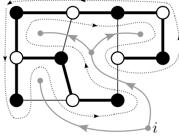
Figure 6.2: Dual graph G^* (solid black), oriented spanning tree T of \vec{G} whose edges are oriented away from vertex i (grey), corresponding spanning tree T^* of G^* (thick edges of G^* ); going around T^* is represented by a dotted line.
