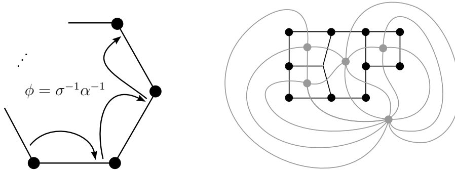
Figure 1.2: Left : the face permutation \phi . Right : a ribbon graph (in black) and its dual (in grey).
