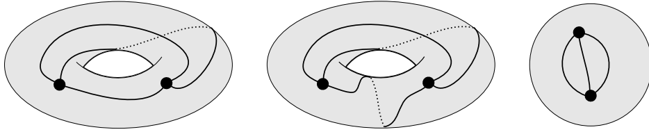
Figure 1.1: The first and the second ribbon graphs are isomorphic. The third one is not isomorphic to the first two, but their underlying graphs are.
