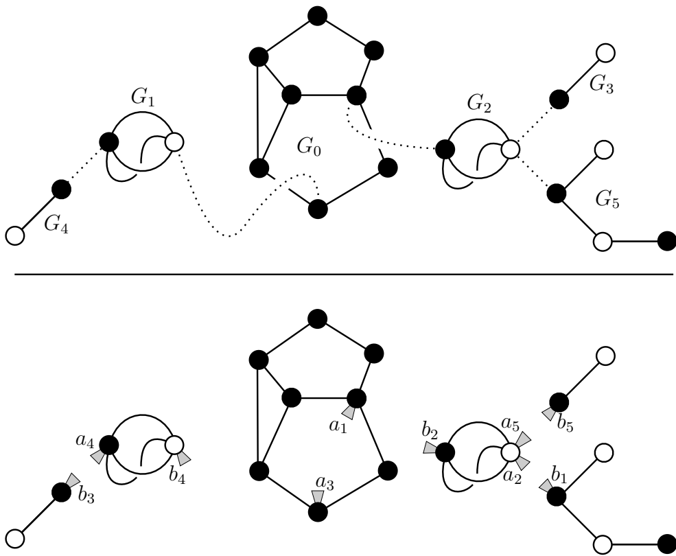
Figure 7.2: An admissible joining (top) and the corresponding sequence of markers (bottom) produced by Algorithm 1.
