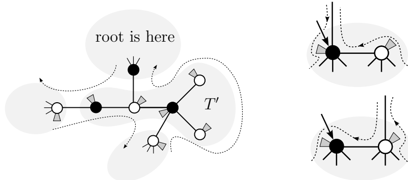
Figure 5.3: Left: going around T , we visit parts of the boundary of a subtree T' in the same order as just going around T' ; the dotted lines represent the tour around T . Right: induced rooting of a subtree T' .
