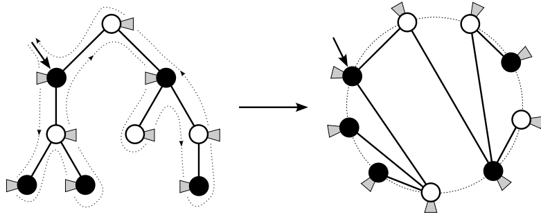
Figure 5.5: Embedding of a tree T with vertices on a circle. The counter-clockwise circular order of vertices on the circle is given by [\pi(T)] .
