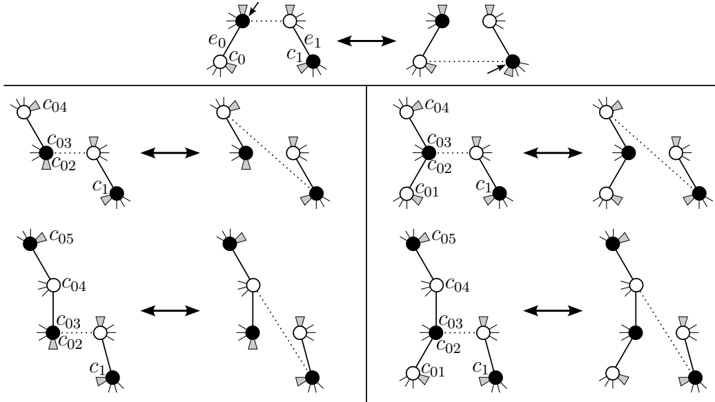
Figure 5.8: Flips preserving [\pi(T)] . In each case the dotted edges are e on the left and e' on the right.
