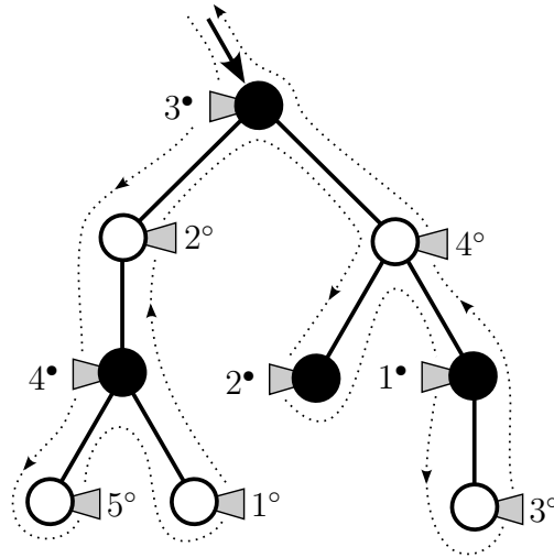
Figure 5.1: Computing the prefix-postfix marking (and sequence) of a tree.
