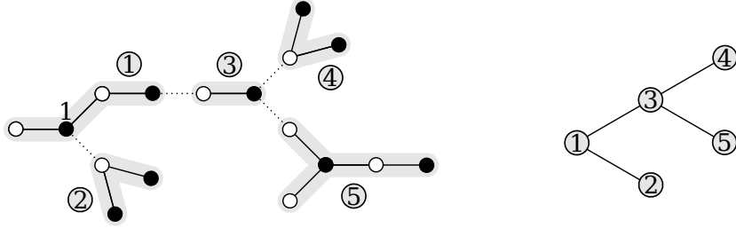
Figure 3.5: Left: a degenerate tree G \in \mathcal{D} with t = 5 constituent positive trees, which are shaded in grey. Their labels are circled. Zero-weight edges are dotted. Black vertex number 1 is in the positive tree number 1. Note that for every zero-weight edge e in G , the black extremity of e is in the same connected component of G - e as the black vertex number 1. Right: the corresponding tree T .
