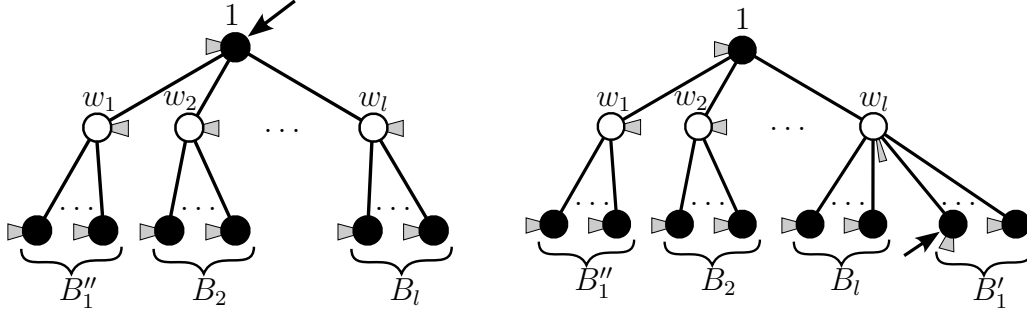
Figure 5.7: Trees T_0 positive at (L; L') and satisfying [\pi(T_0)] = c_0 .
