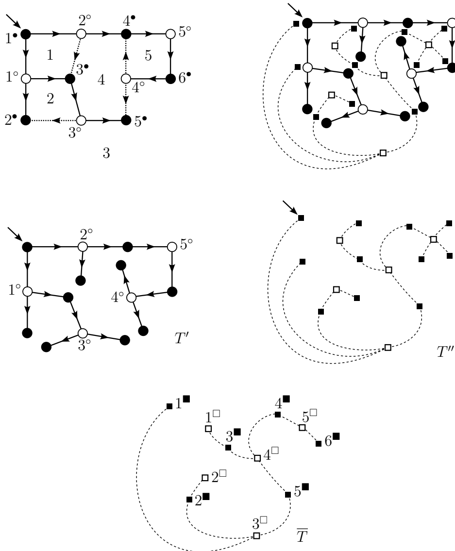
Figure 6.7: Steps of the map \psi . First row, left : a rooted labeled vertex-colored map with orientation corresponding to some spanning tree (dotted edges do not belong to the tree). First row, right : applying Bernardi bijection. Second row : resulting trees T' and T'' . Third row : the tree \bar{T} constructed from T'' .
