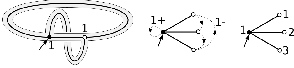
Figure 3.4: A ribbon graph from \mathcal{E}_{1,1,1}^{*,root} , one of its corresponding C-decorated trees from \mathcal{CT}_{1,3,1,1} , and one of the rooted labeled trees from \mathcal{E}_{0,1,3}^{*,root} corresponding to this C-decorated tree.
