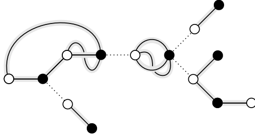
Figure 2.3: A vertex-bicolored ribbon graph which has degenerated into a disconnected graph with 4 components. The bridges of zero length are dashed. They connect the components together into a tree-like structure.
