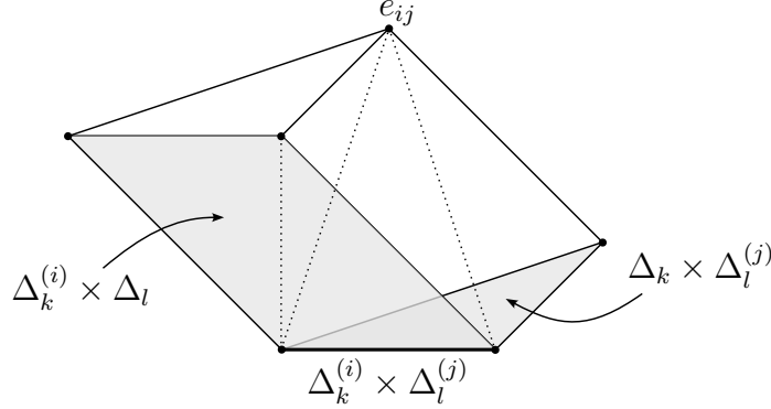
Figure 5.2: Recursive construction of triangulations (the particular case of a triangular prism \Delta_2 \times \Delta_1 is shown).
