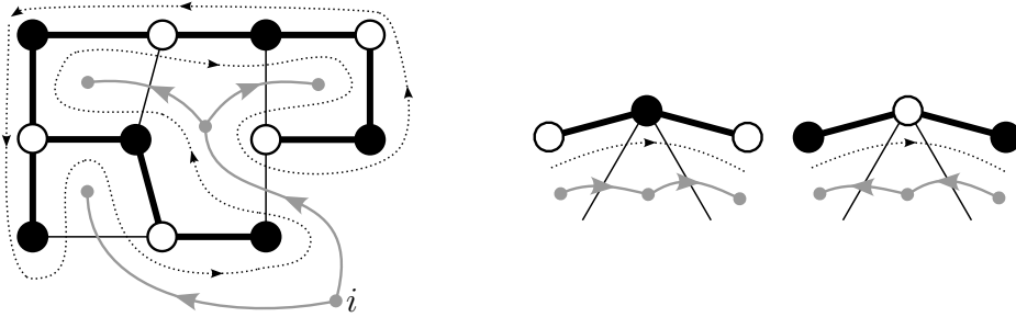
Figure 6.6: Left : dual graph G^* (solid black), oriented spanning tree T of \vec{G} whose edges are oriented away from vertex i (grey), corresponding spanning tree T^* of G^* (thick edges of G^* ); going around T^* is represented by a dotted line. Right : local picture of going around T^* (and T ).
