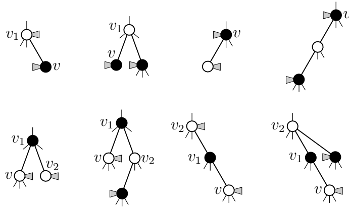
Figure 5.4: Possible configurations of two consecutive markers.
