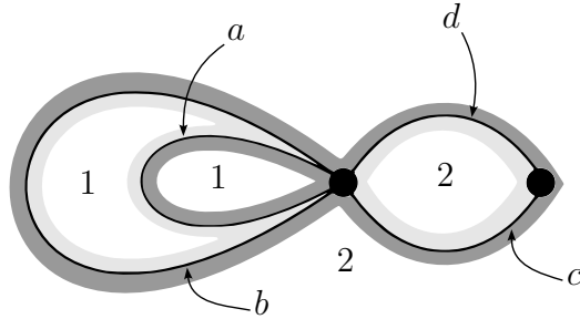
Figure 1.3: Computing the counting function of a face-bicolored ribbon graph.
