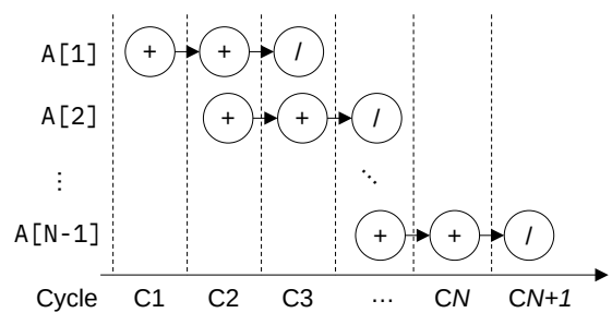
Figure 3.4 – Loop pipelining in HLS overlaps multiple iterations of a loop, starting a new iteration every II cycles (here II=1), provided there is no dependence between them.
