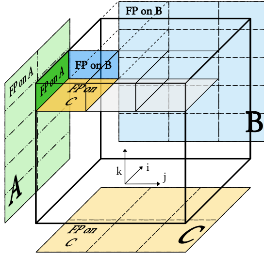
Figure 7.1 – Tiled matrix product, and footprint of a tile on the matrices. Each footprint “patch” is composed of multiple contiguous rows or columns, but none of the patches are entirely contiguous in memory.
