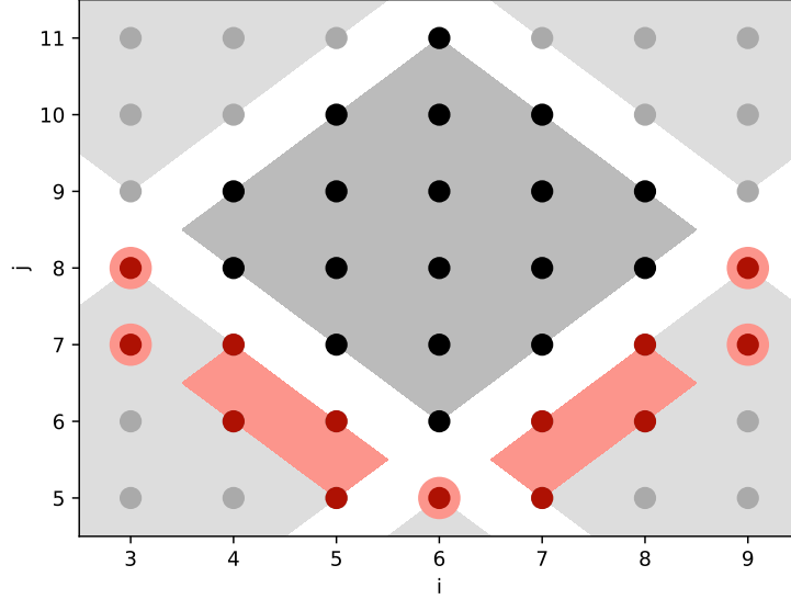
Figure 7.8 – Coincidence between MARS computed with the uniform dependence method, and those computed with the affine method.
