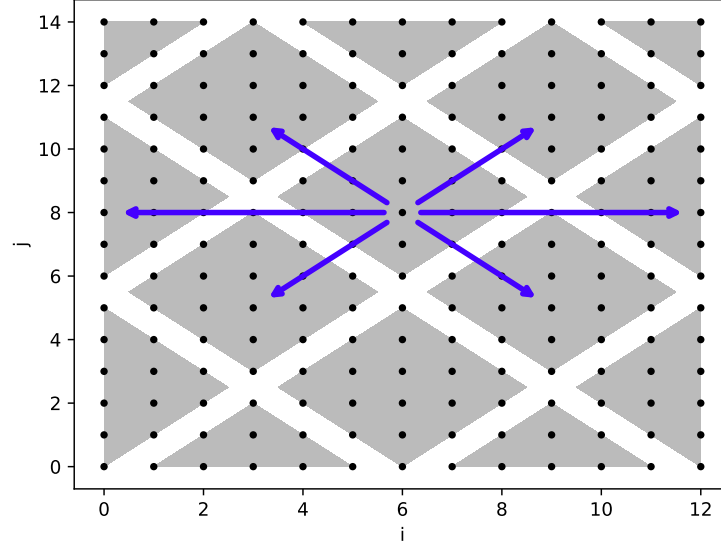
Figure 7.6 – Consumer tiles of array \mathcal{A} with Jacobi 1D dependences, sharing their footprint with tile T(\vec{t}) .
