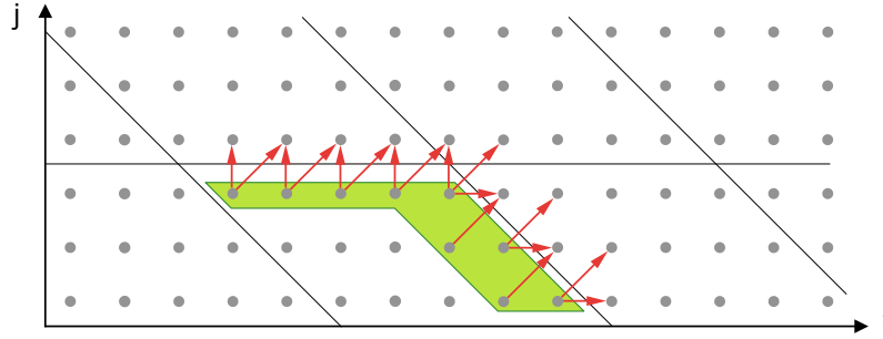
Figure 3.10 – Flow-out set of a tile with a Smith-Waterman dependence pattern. Dependencies pointing to other tiles are shown producer to consumer:.
