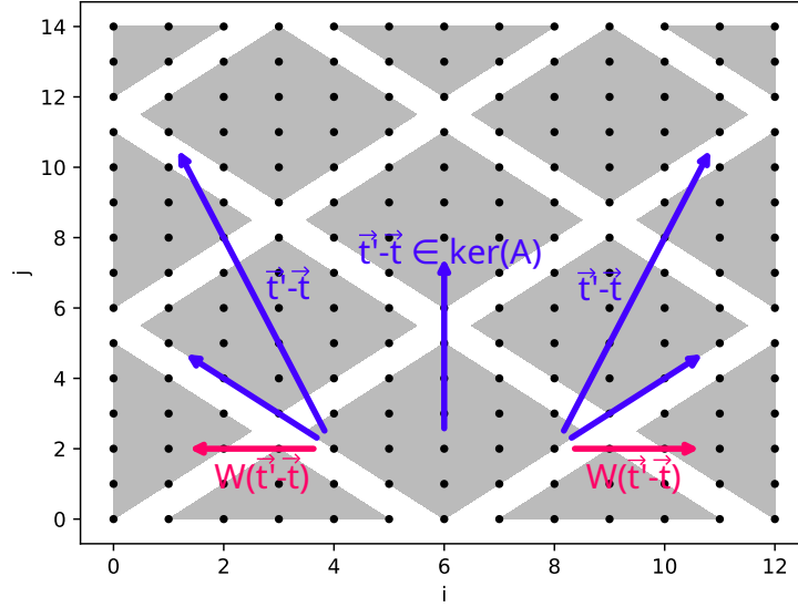
Figure 7.3 – Some consumer tiles of one tile T(\vec{t}) with a single dependence B(i, j) = (i) , and the projection W(\vec{t}' - \vec{t}) on a supplementary of \ker(A) . There are a finite number of such projected vectors, and they are constant.
