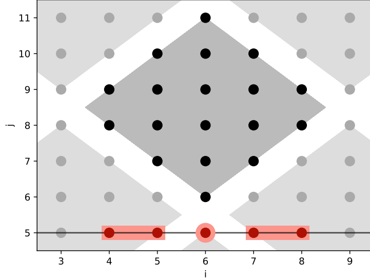
Figure 7.4 – MARS obtained with a single affine dependence B(i, j) = (i) .
