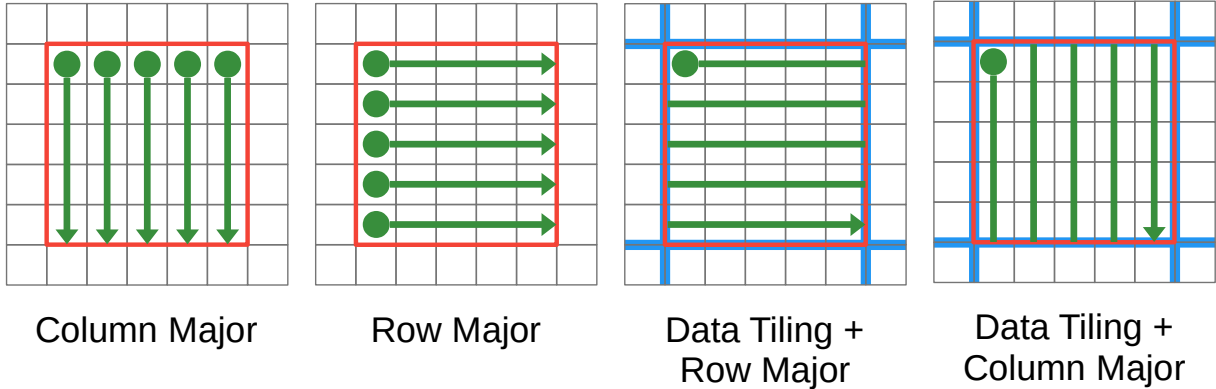
Figure 4.2 – Memory layouts (non-tiled and tiled) for a 2-dimensional data space, and access patterns for a tile. Each dot is the start of a burst access, that spans until the arrow tip. Data tiling layouts enable a single burst access per tile instead of one per row/column.
