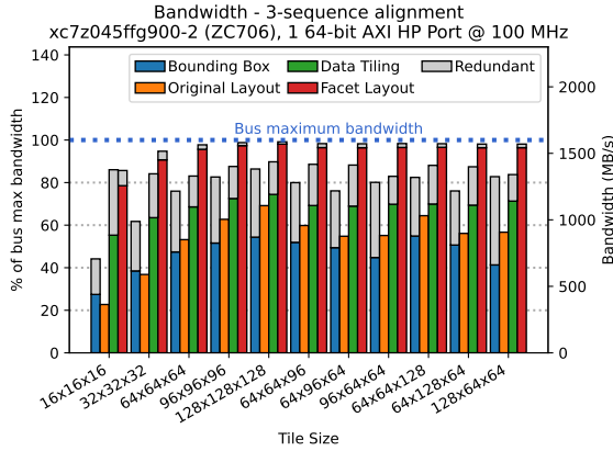
(a) sw3d
