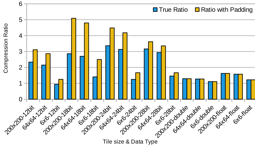
Figure 6.11 – Compression ratio vs. data type and tile size for jacobi1d
