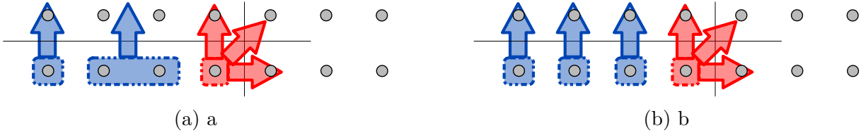
Figure 5.1 – Sets of iterations for Smith-Waterman matching single-producer, atomicity properties, but not maximality. Maximality forces the search for a non-trivial solution
