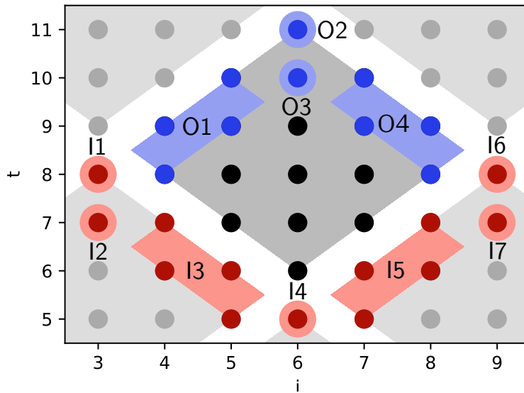
Figure 6.5 – MARS: Groups of points within a tile which data is contiguous in global memory. In blue, the MARS produced by the center tile (O1 to O4); in red, the MARS consumed by that same tile (I1 to I7).
