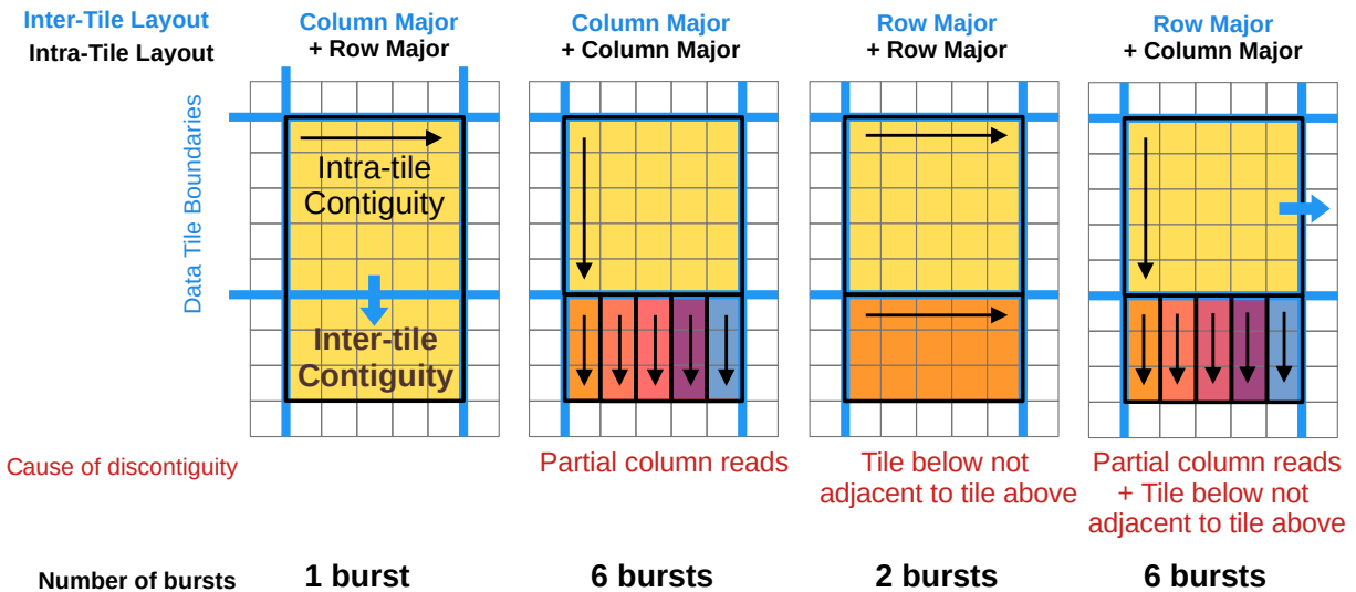
Figure 4.7 – The four possible data layouts for a 2-dimensional array in tiled data layout (inter-tile + intra-tile layouts), and the number of bursts needed to read a tile and part of the tile below it. Only one layout allows a single burst spanning both tiles.
