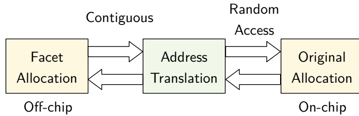
Figure 3.6 – Changing layouts is necessary to get both contiguity and parallelism.
