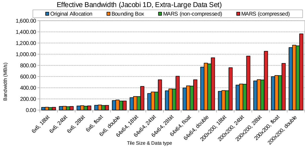
(a) jacobi-1d
