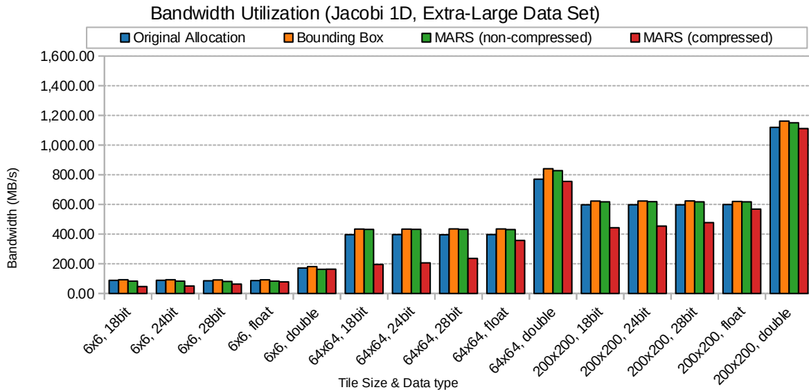
(a) jacobi-1d
