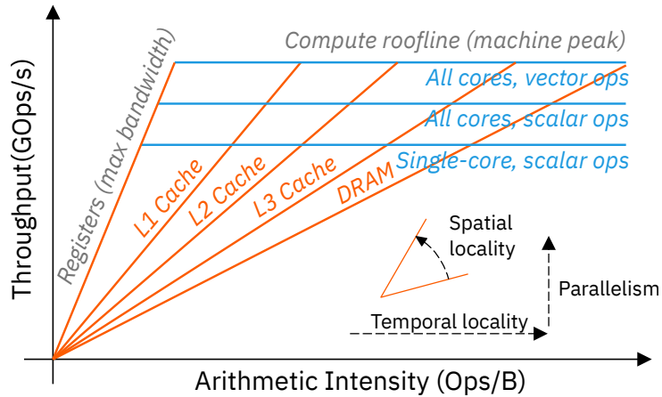
Figure 3.1 – Roofline model
