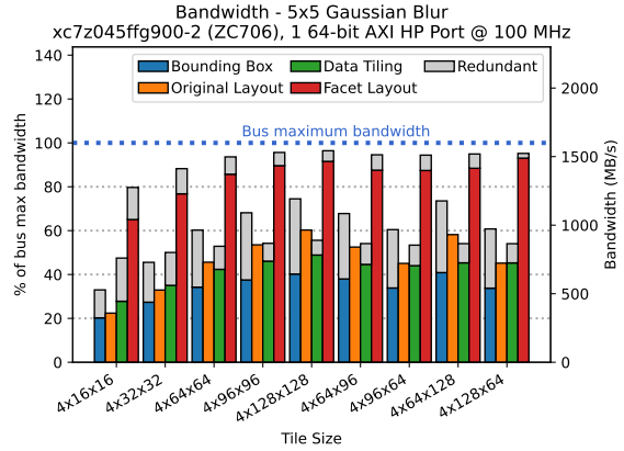
(b) gaussian
