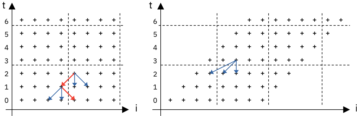
Figure 3.8 – Rectangular tiling (cutting with a family of hyperplanes \mathcal{H}_i : i = 4k, k \in \mathbf{N} and \mathcal{H}_t : t = 3p, p \in \mathbf{N} ) is illegal on the left, and becomes legal on the right after time skewing.
