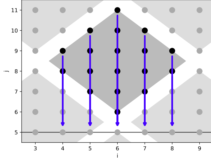
Figure 7.2 – Footprint of one tile with a single affine dependence B(i, j) = (i) . The one-dimensional destination space is shown as a continuous line.
