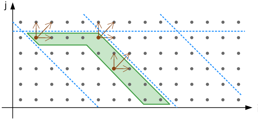
Figure 5.2 – Flow-out set for a skewed tile of a Smith-Waterman kernel. The arrows correspond to the dependence pattern (PRDG).
