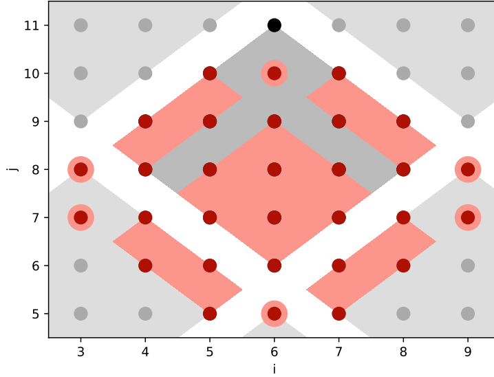
Figure 7.7 – MARS for uniformly intersecting dependences (Jacobi 1D)
