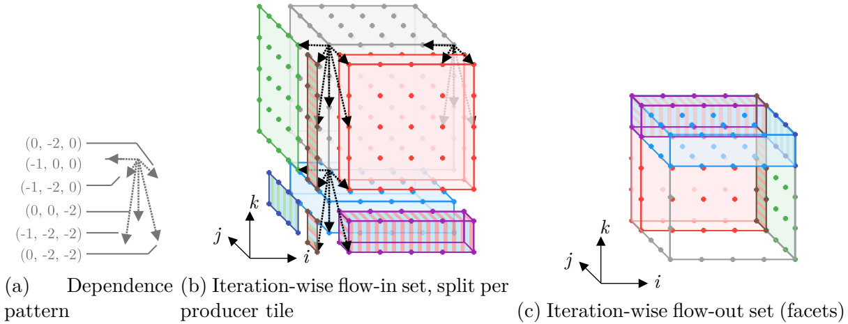
Figure 4.3 – An instance of flow-in and flow-out sets. The flow-out set is the union of thicker versions of the tile faces (facets), while the flow-in set is composed of an union of either whole or partial facets. Some flow-in sets are adjacent in the iteration space; CFA reflects this adjacency in memory.
