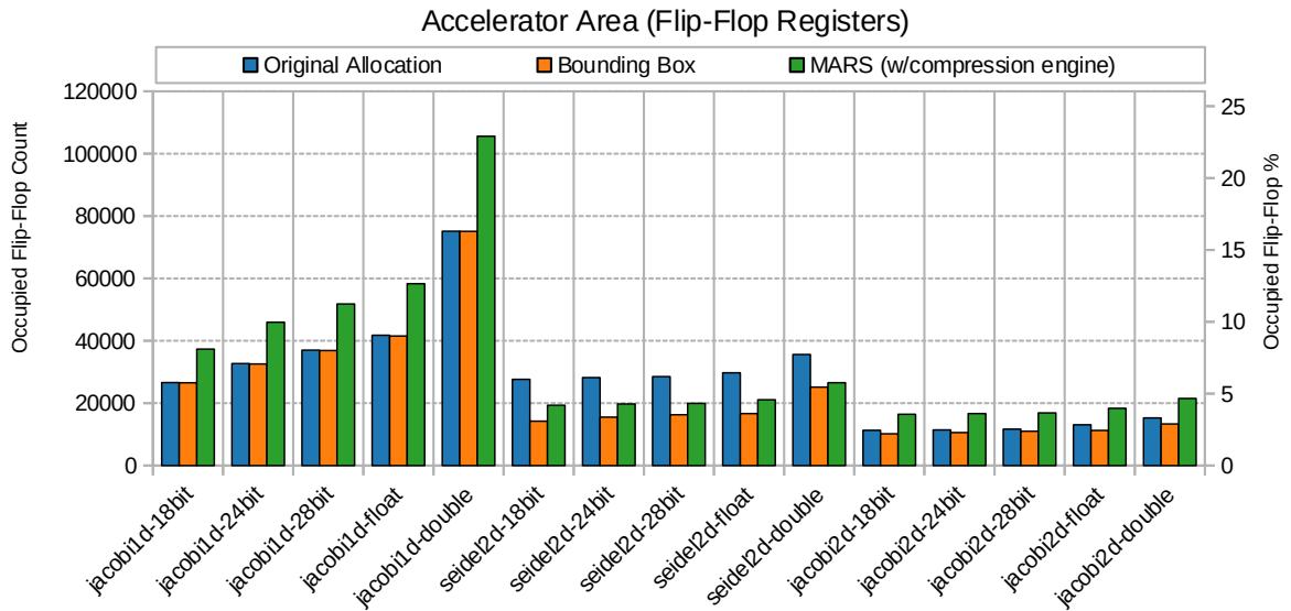
(b) Flip-flops
