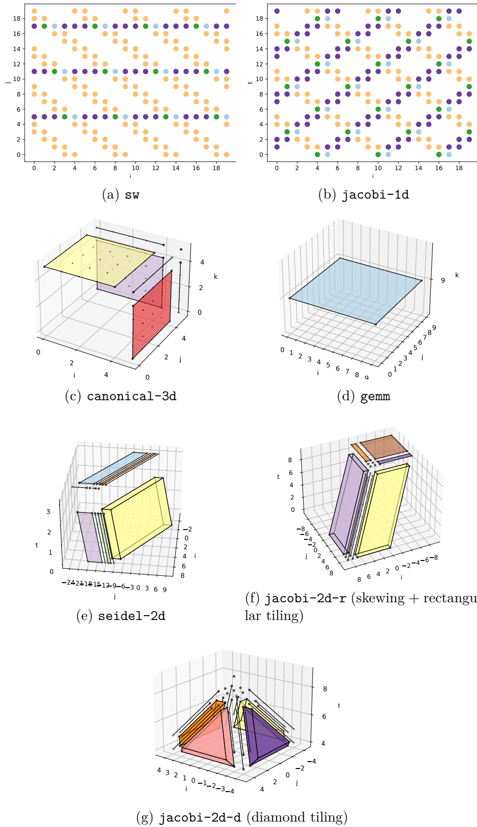
Figure 5.5 – Visualization of MARS-generated using the MARS calculator.
