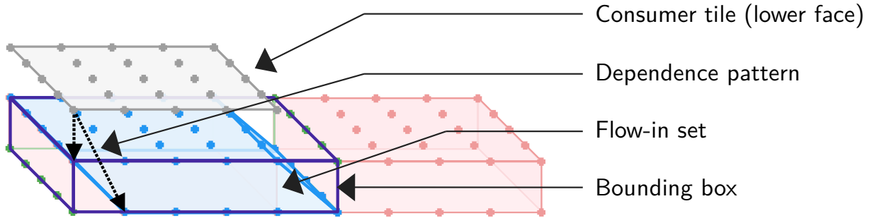
Figure 4.10 – Taking a rectangular over-approximation of the actual flow-in set incurs redundant reads. Contiguous data (facets) are in red: an over-approximation may be necessary to preserve access contiguity.
