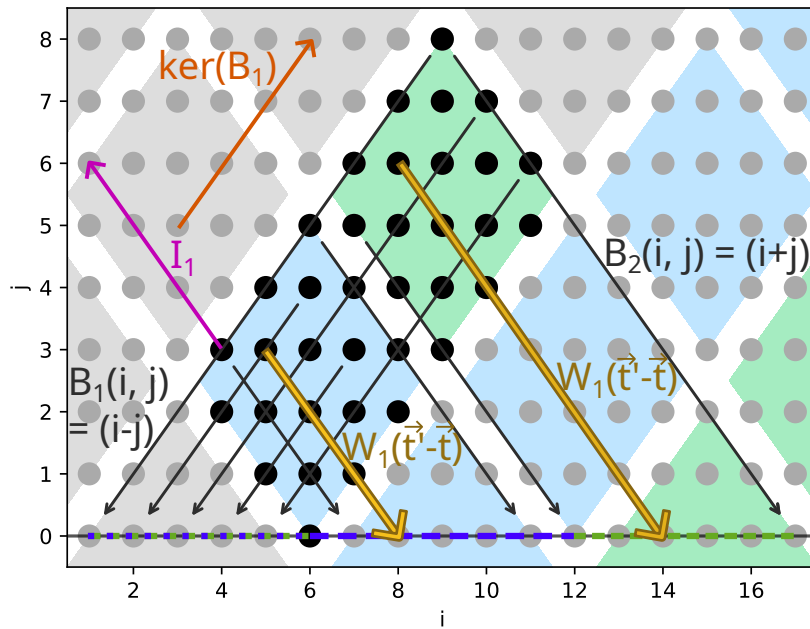
Figure 7.9 – Non-uniformly intersecting dependences do not guarantee that the vectors W_i(\vec{t}^i - \vec{t}^j) do not depend on \vec{t}^i , i.e. each tile's footprint is not necessarily a translation of another tile's footprint.
