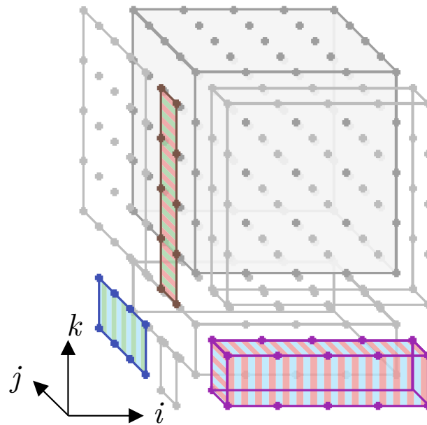
Figure 4.6 – Flow-in iterations from second-level neighbors of an iteration tile. CFA places in memory each data tile containing a slab next to a fully consumed data tile to read both in the same burst.
