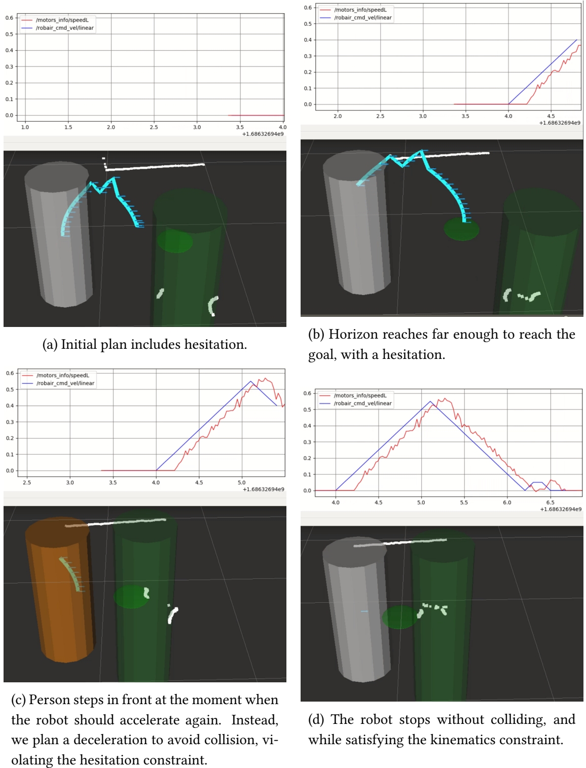
Figure 5.12: Interrupting a hesitation in order to avoid collision. Top: past command velocities issued at 10\text{hz} (blue) and odometry estimated at 40\text{hz} (red) in \text{m.s}^{-1} , plotted w.r.t. time (s). Bottom: visualisation of the planned velocity w.r.t. position. Robot (gray or orange cylinder), person (green cylinder). Orange cylinder indicates the robot is executing a motion that does not comply with all prosody constraints. The robot goal position is at the center of the green disk.
