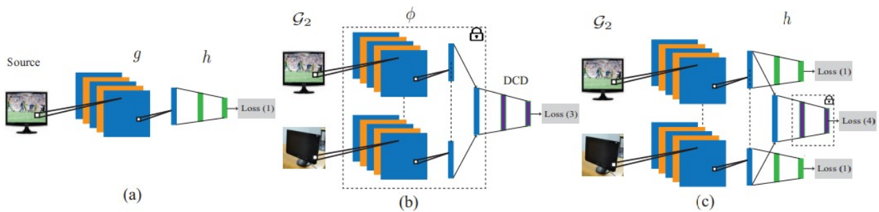
Figure 3.21: The training of FADA in three stages. (a) Features extractor g and label predictor h are trained on the source domain D_s . (b) A domain-class discriminator (DCD) is trained while g is frozen. (c) DCD is frozen while g and h are trained. Figure from [117]
