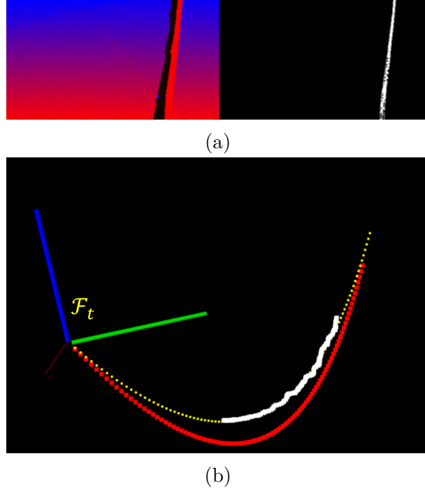
Figure 4.4 – Demonstration of the proposed visual features estimation with eye-in-hand camera setup. (a) Depth image on the left and segmented cable on the RGB image on the right. Depth image is aligned with the RGB image. (b) 3D view: the white points correspond to the cable points which are projected to the tether frame (4.6) and then used to estimate a, b . Fitted parabola in \mathcal{F}_t depicted in yellow after the processing of the cable pointcloud in the world frame composed of: downsampling \rightarrow RANSAC \rightarrow {}^w\mathbf{n} sign check and filtering \rightarrow \alpha, \phi \rightarrow (4.6) \rightarrow least squares fitting and a, b filtering. Red points correspond to some desired shape a^*, b^* . Note that the cable inliers distribution is more dense compared to the eye-to-hand case, but less of the cable is visible in the RGB camera FOV that is limited by the lens and orientation of the camera.
