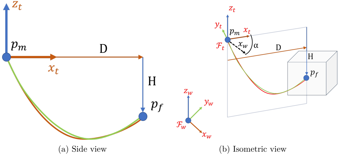
Figure 3.1 – Tether cable (green curve) and its parabola model (red curve): D > 0 , H < 0 in this configuration.
