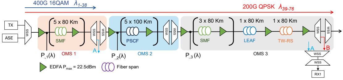
Figure 2.15: Tandem Network Setup
