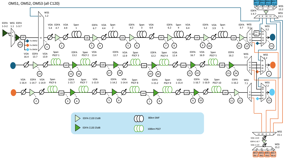
Figure 2.13: Expérimental Setup Description
