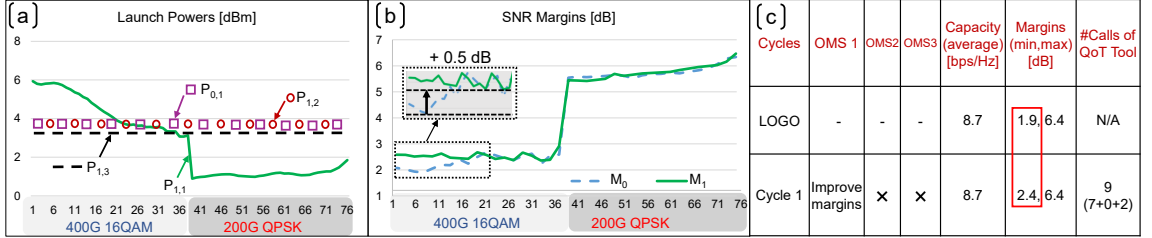
Figure 2.17: Experiment: (a) launch powers P_{j,n} for all services on n^{\text{th}} OMS at Cycle j ; (b) Margins M_j for all services at Cycle j ; (c) Cycles
