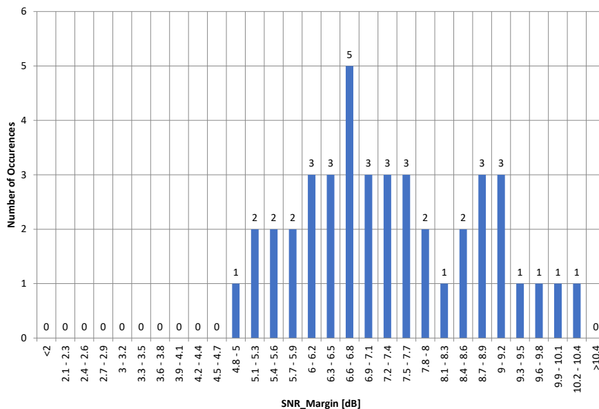
Figure 3.11: Available SNR margins in the network
