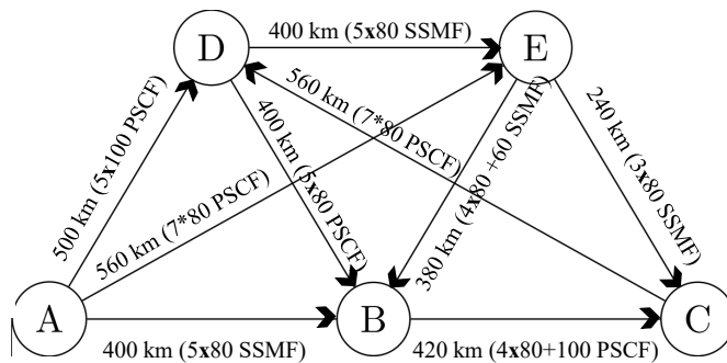
Figure 3.6: Network Topology with 5 nodes
