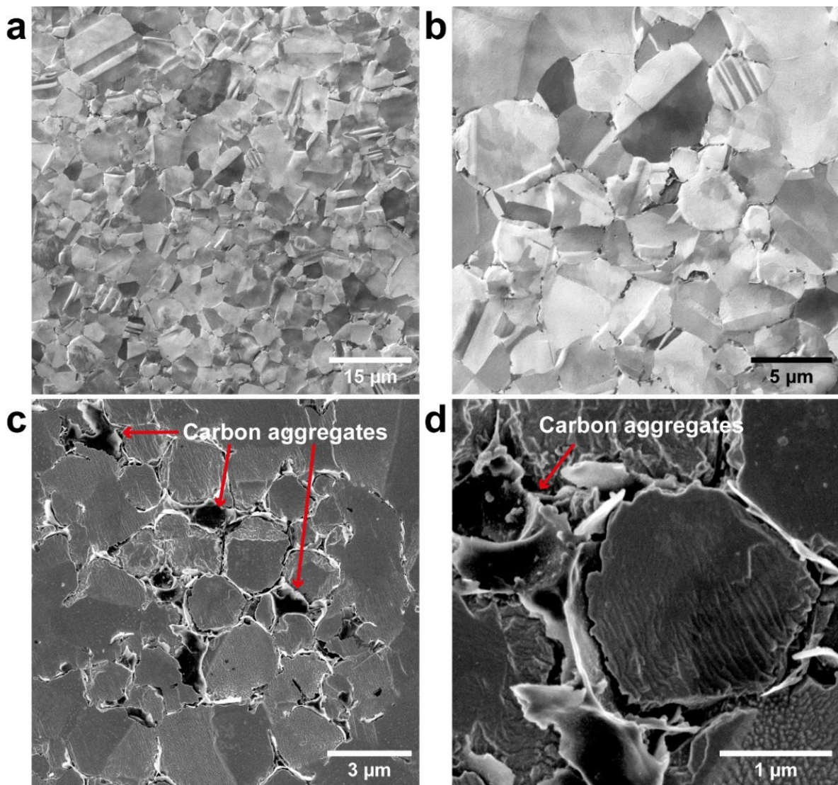
Figure 3.8 – SEM observations of the microstructure of rCu200C@2.00%(900°C - 100MPa) using ICCI: a microstructure of the sample and b its associated magnification, c observation of a grain boundary and d its associated magnification
