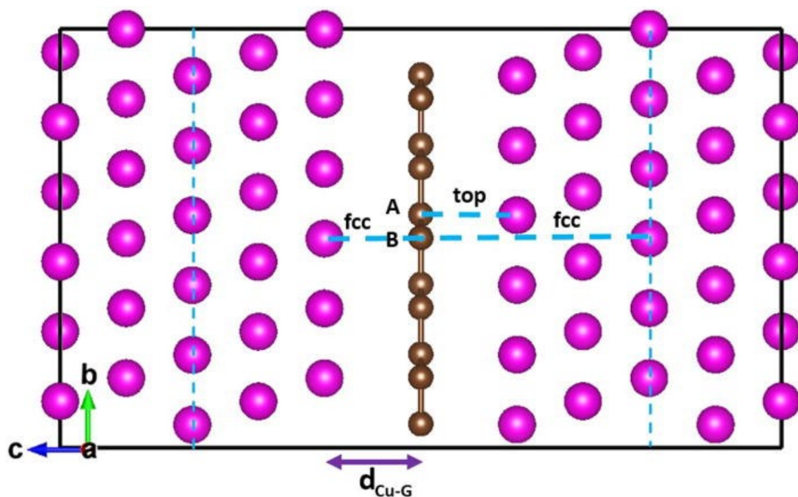
Figure 1.15. Geometry of the Cu/G/Cu model with d_{\text{Cu-G}} representing the Cu–G distance. Top–fcc configuration of graphene above the Cu 111 surface with A and B representing sub-lattice sites above the Cu atom at first and third layers, respectively. The pink and brown colored spheres represent Cu and C atoms, respectively. [127]
