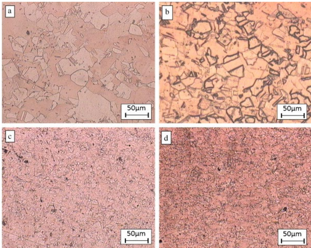
Figure 1.6. Optical micrographs of the (a) as-annealed, (b) 1-pass ECAR'ed, (c) 7-pass ECAR'ed and (d) 10-pass ECAR'ed specimens. [18]
