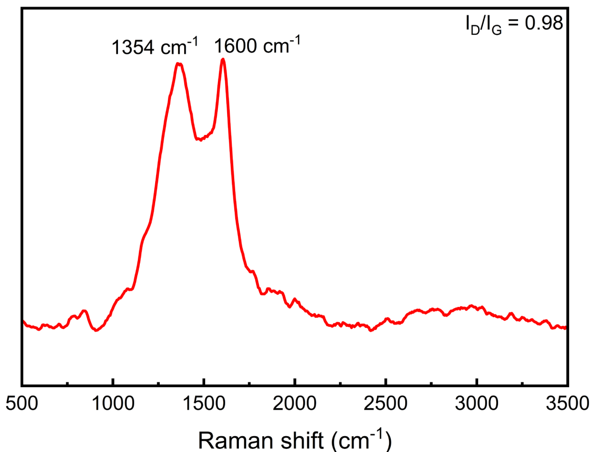
Figure 2.16 – Raman spectra of the rCu200C@2.00% powder after graphitization at 1000°C
