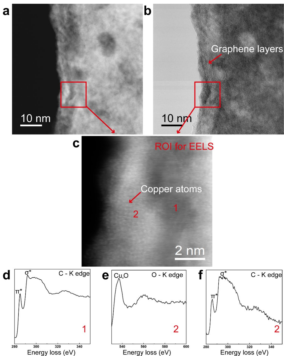
Figure 2.14 – TEM observations and EELS analysis of the Cu@2.00% powder: a HAADF observation, b bright field observation, c ROI for EELS analysis the numbers 1 and 2 denotes the location of gathered specific EELS, d EELS of the zone 1, e and f EELS of the zone 2
