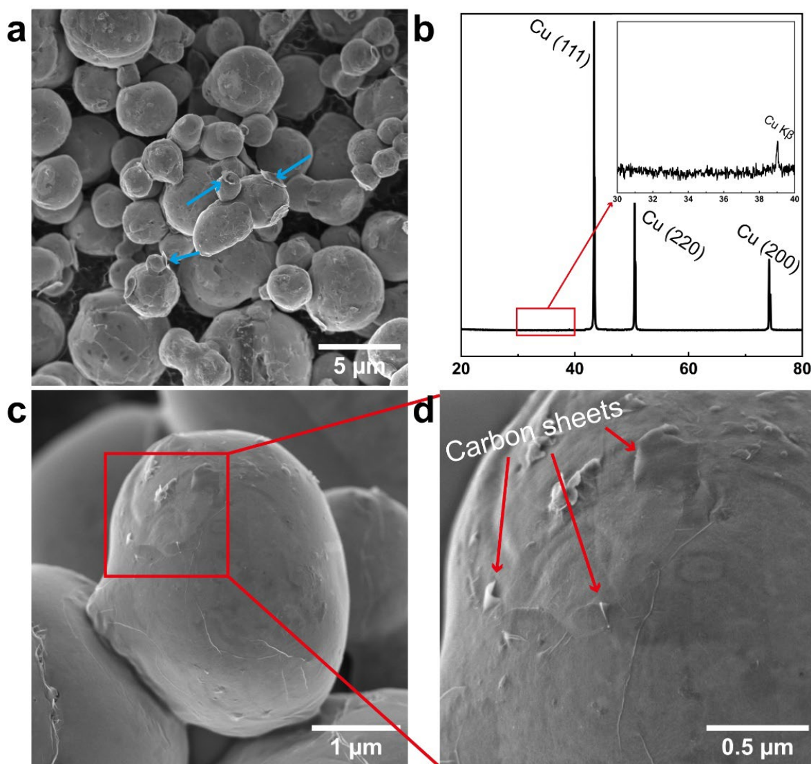
Figure 2.15 – General characterization of the \text{rCu200C@2.00\%} powder after graphitization at 1000^{\circ}\text{C} : a SEM image the particles where the carbon is pointed by blue arrows, b the associated XRD diagram, c SEM image showing a particle still covered carbon sheet and d the associated magnification
