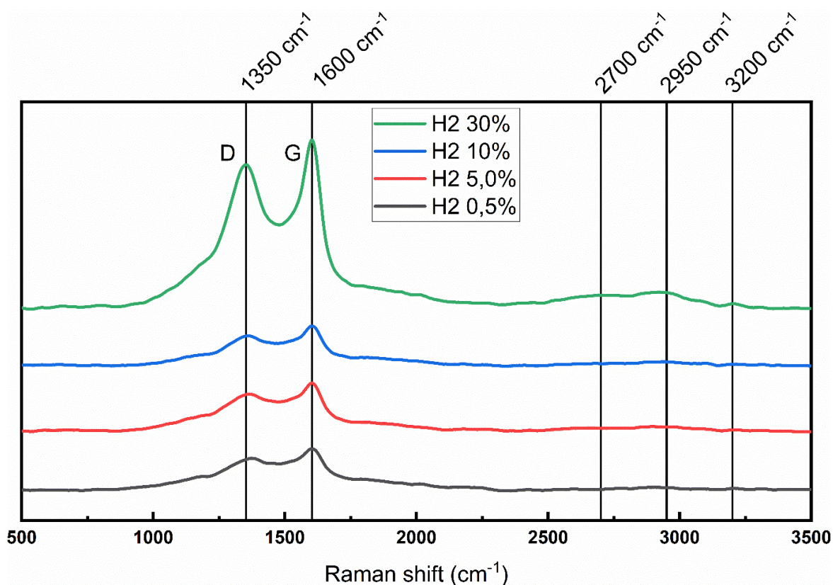
Figure 2.22 – Stacked Raman spectra of the rCu@0.65\% powder with varying hydrogen proportions: H_2 30 vol% in green, H_2 10 vol% in blue, H_2 5 vol% in red and H_2 0.5 vol% in grey
