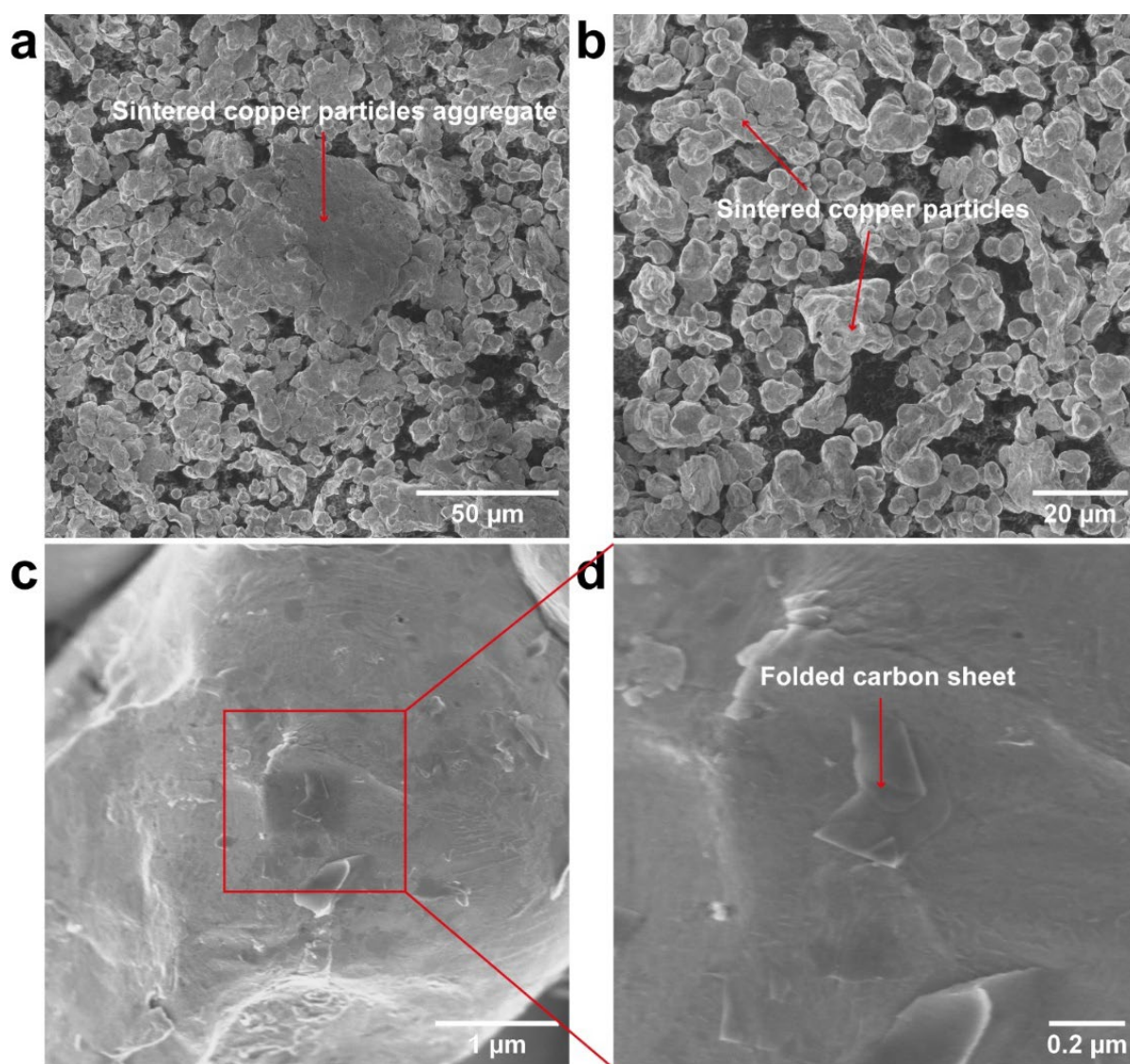
Figure 2.23 – General SEM characterization of the \text{rCu}_{200}\text{C}@0.65\% after 60min
