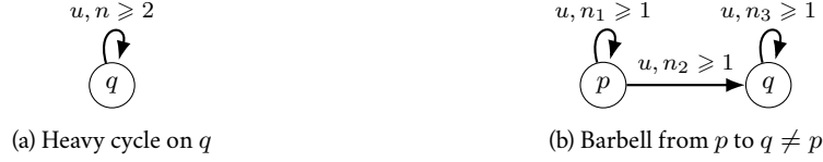
Figure 4.48: Patterns that create unboundedness in a trim \mathbb{N} -automaton.
