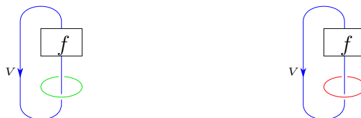
Figure 3.1: The graph on the left is a ribbon graph T in S^2 \times S^1 where the green circle represents the topology of S^2 \times S^1 . The graph on the right is a bichrome graph in S^3 which after surgery on the red circle produces the graph on the left.
