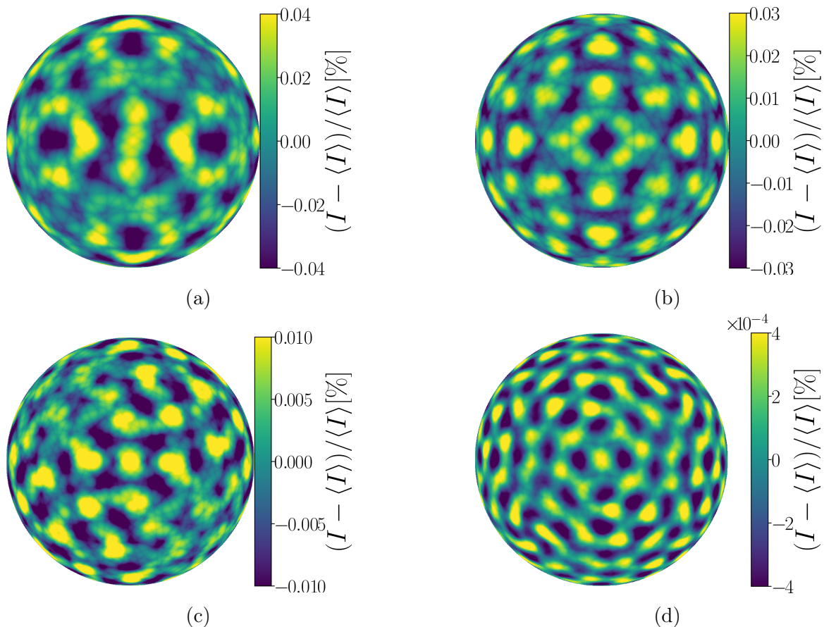
Figure 5.3 – Orthogonal projections of intensity distributions for designs T72 (a), 13t96 (b), 14t108 (c), 21t240 (d). The more laser beams, the higher is the peak mode and the better is the irradiation uniformity.
