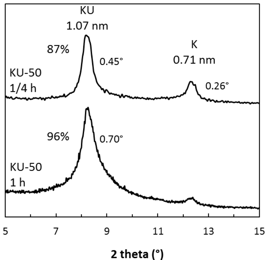
Figure. I.2. X-ray diffraction patterns of the (001) reflection of kaolin mechanically ground together with 50 m% (KU-50) solid urea for (1/4, 1 h). The degree of intercalation (%), the FWHM values of the reflections (°) and d-values (nm) of the expanded and non-expanded kaolinite are indicated. KU-50 was as ground sample.
