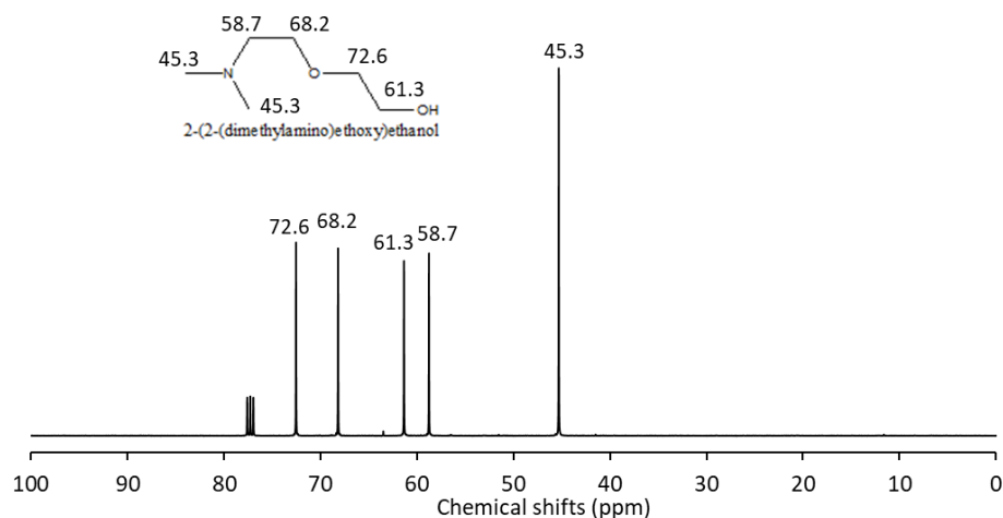
Figure IV.7. ^{13}\text{C} NMR spectra for DAEE molecule.
