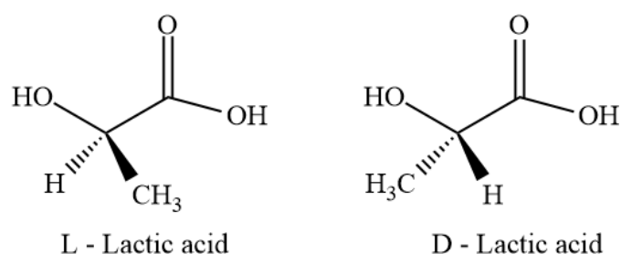
Figure 1.17. Different isomeric forms of lactic acid [148].
