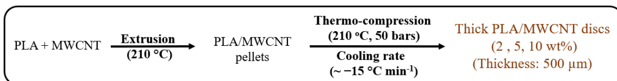
Figure 2.1. Melt-blending process for thick samples made with PLA/MWCNT preparation.
