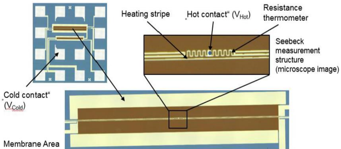
Figure 2.22. VDP chip setup with heater and resistance thermometer on the larger membrane [25].
