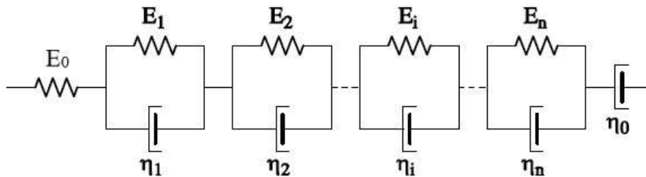
Figure 2.23. The generalised Kelvin-Voigt Model.
