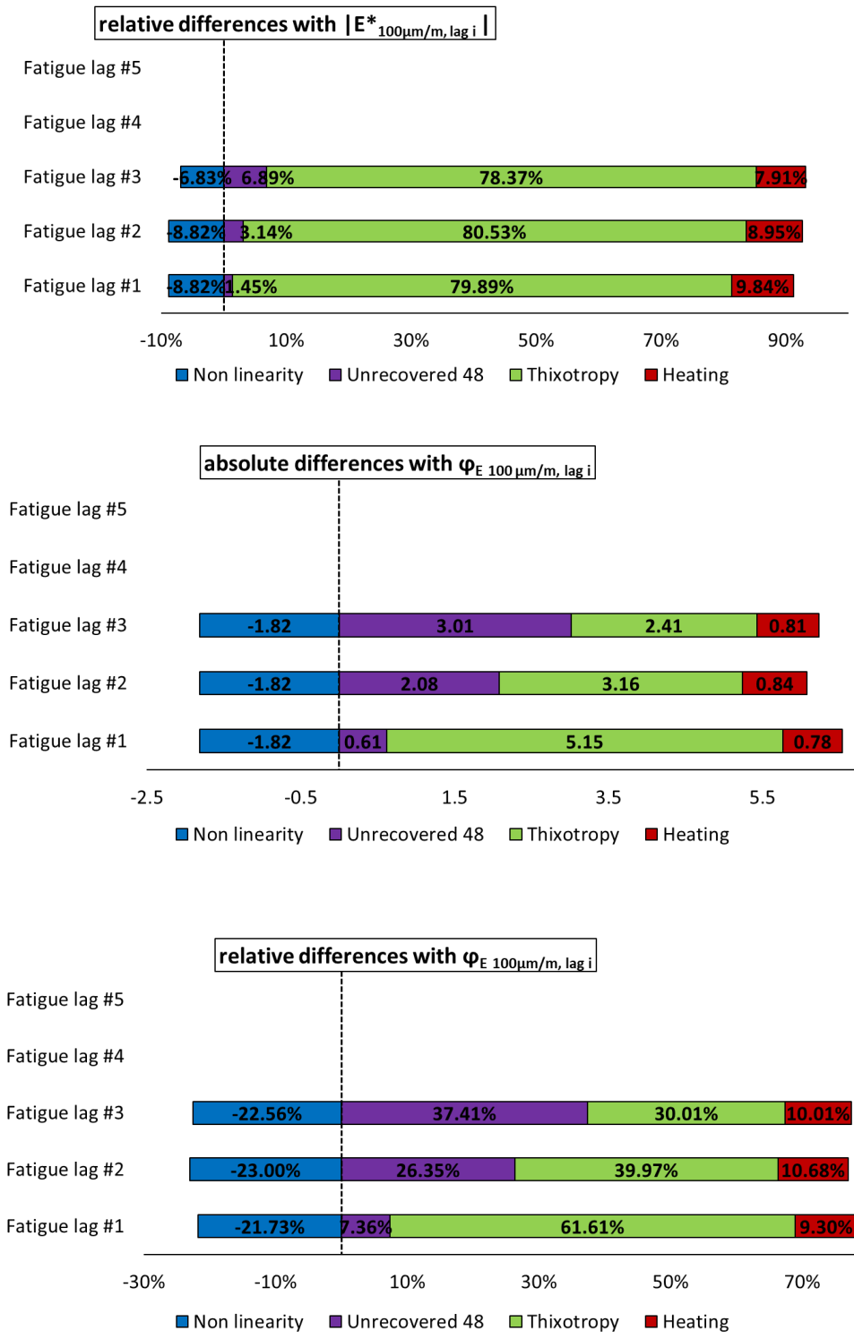
Figure 3.1.33. Quantification of different absolute and relative contributions to |E^*| and \varphi_E evolutions for mix 70/100 – 5, calculated using the envelope line for the first fatigue lag.
