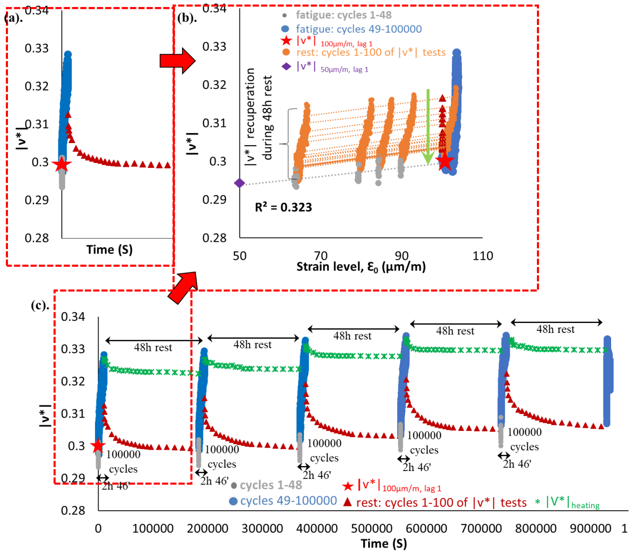
Figure 5.11. PFRT results obtained for mix 40/60 – 7: |v^*| evolution during fatigue lags and recovery periods. The red star indicates the value of |v^*| estimated at 100 \mu\text{m}/\text{m} at the beginning of the first fatigue lag, purple diamond indicates the value of |v^*| estimated at 50 \mu\text{m}/\text{m} , green asterisks show values of \Delta|v^*_{\text{heating}}| and brown triangles indicate values of |v^*| estimated at 100 \mu\text{m}/\text{m} , after 48 hours of recovery, with non-linearity envelope.
