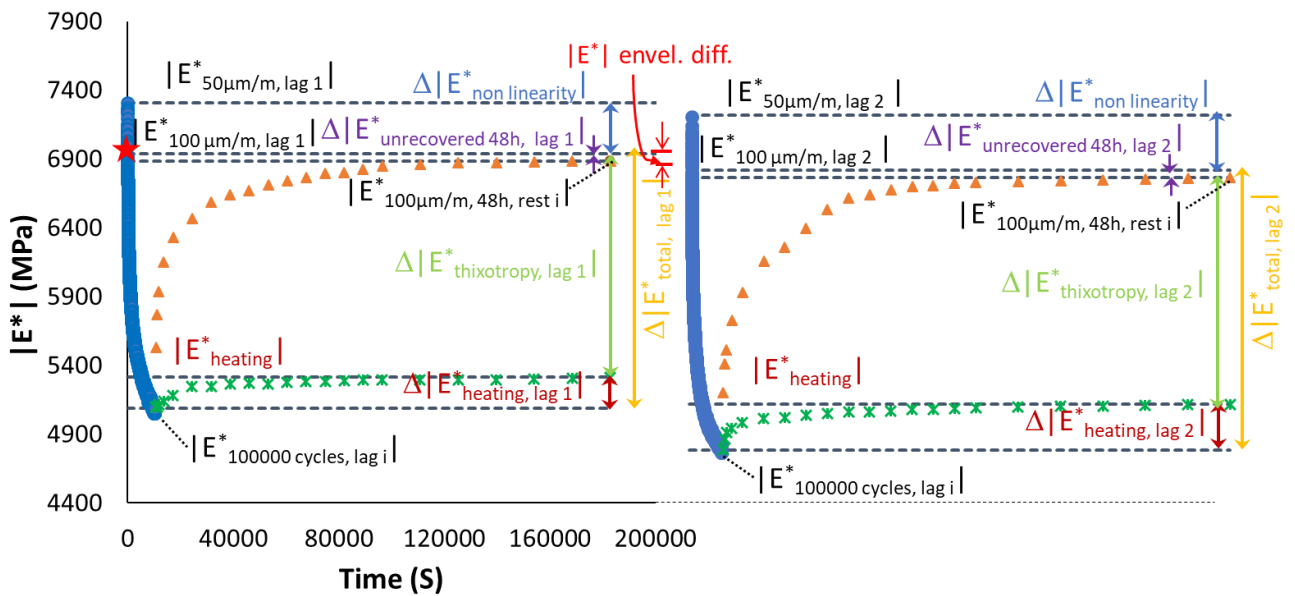
Figure 5.18. Quantification of different contributions to |E^*| evolution, for the first two fatigue lags for mix 40/60 - 7: different envelope line is used for each fatigue lag.
