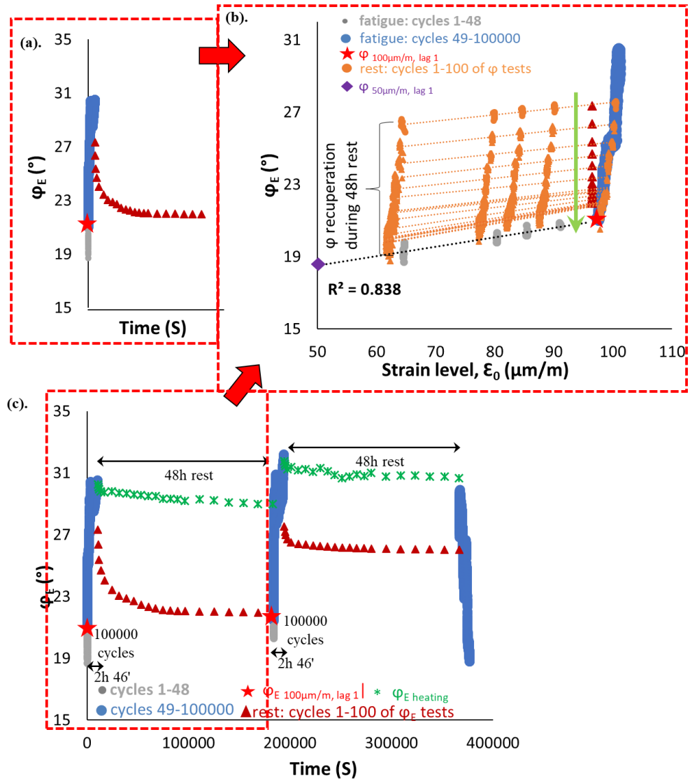
3.1.9. PFRT results obtained for mix 70/100 – 3: (a) \phi_E as a function of time during the first fatigue lag and rest period (b) \phi_E as a function of applied strain amplitude during the first fatigue lags and the short complex modulus tests performed within its following rest periods; (c) \phi_E as a function of time during the two fatigue lags and rest periods (Red stars indicate values of \phi_E estimated at 100 \mu\text{m/m} at the beginning of fatigue lag, green asterisk shows values of \Delta\phi_{\text{heating}} as influence of self-heating and brown triangles indicate values of \phi_E estimated at 100 \mu\text{m/m} for each short complex modulus test during rest (all these values were obtained using non-linearity envelopes, as shown in (b) for the first fatigue lag and rest period).
