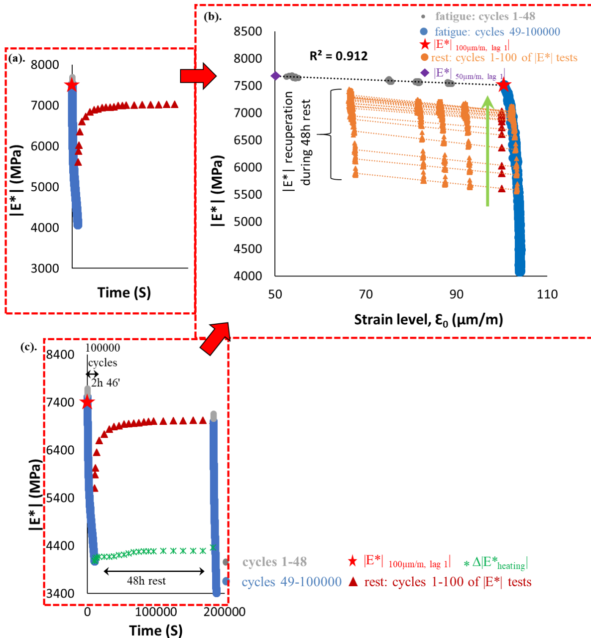
Figure 5.14. PFRT results obtained for mix 70/100 - 1: |E^*| evolution during fatigue lags and recovery periods. The red star indicates the value of |E^*| estimated at 100 \mu\text{m/m} at the beginning of the first fatigue lag, purple diamond indicate the value of |E^*| estimated at 50 \mu\text{m/m} , green asterisks show values of \Delta|E^*_{\text{heating}}| ( E^* corrected from self-heating during rest periods, explained afterwards in this chapter) and brown triangles indicate values of |E^*| estimated at 100 \mu\text{m/m} , after 48 hours of recovery, with non-linearity envelope.
