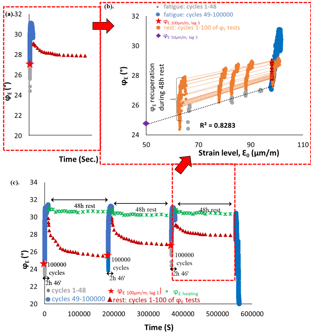
3.1.27. PFRT results obtained for mix 70/100 – 5: (a) \phi_E as a function of time during the third fatigue lag and rest period (b) \phi_E as a function of applied strain amplitude during the third fatigue lags and the short complex modulus tests performed within its following rest periods; (c) \phi_E as a function of time during the three fatigue lags and rest periods (Red stars indicate values of \phi_E estimated at 100 \mu\text{m}/\text{m} at the beginning of fatigue lag, green asterisk shows values of \Delta\phi_E heating as influence of self-heating and brown triangles indicate values of \phi_E estimated at 100 \mu\text{m}/\text{m} for each short complex modulus test during rest (all these values were obtained using non-linearity envelopes, as shown in (b) for the first fatigue lag and rest period).
