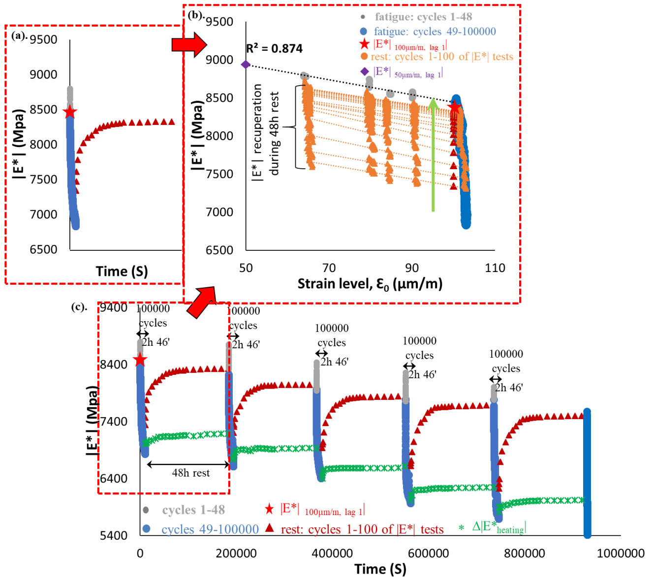
3.1.43. PFRT results obtained for mix 40/60 – 4: (a) |E^*| as a function of time during the first fatigue lag and rest period (b) |E^*| as a function of applied strain amplitude during the first fatigue lags and the short complex modulus tests performed within its following rest periods; (c) |E^*| as a function of time during the five fatigue lags and rest periods [Red stars indicate values of |E^*| estimated at 100 \mu\text{m}/\text{m} at the beginning of fatigue lag, green asterisk shows values of \Delta|E^*_{\text{heating}}| as influence of self-heating and brown triangles indicate values of |E^*| estimated at 100 \mu\text{m}/\text{m} for each short complex modulus test during rest (all these values were obtained using non-linearity envelopes, as shown in (b) for the first fatigue lag and rest period)].
