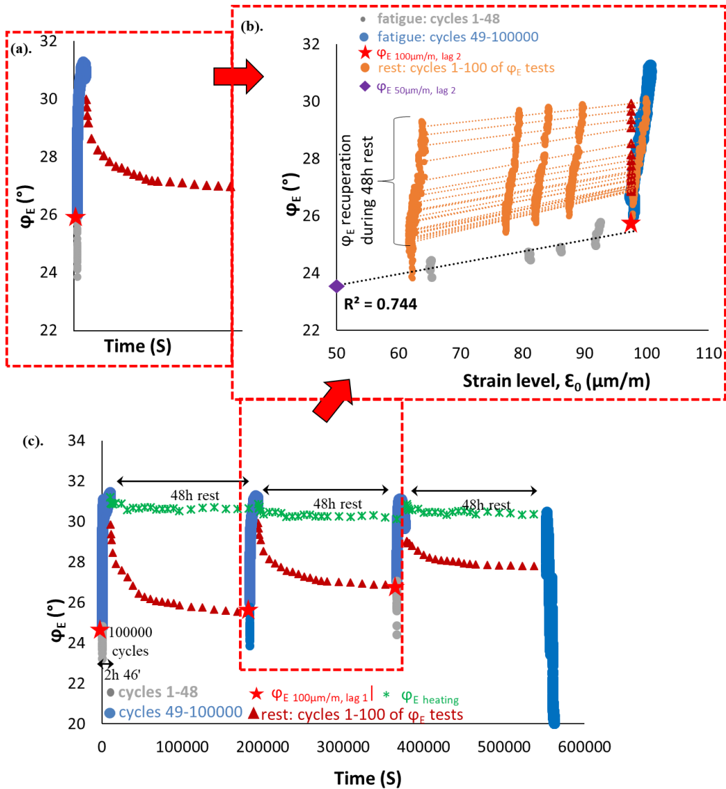
3.1.26. PFRT results obtained for mix 70/100 – 5: (a) \varphi_E as a function of time during the second fatigue lag and rest period (b) \varphi_E as a function of applied strain amplitude during the second fatigue lags and the short complex modulus tests performed within its following rest periods; (c) \varphi_E as a function of time during the three fatigue lags and rest periods (Red stars indicate values of \varphi_E estimated at 100 \mu\text{m}/\text{m} at the beginning of fatigue lag, green asterisk shows values of \Delta\varphi_{E \text{ heating}} as influence of self-heating and brown triangles indicate values of \varphi_E estimated at 100 \mu\text{m}/\text{m} for each short complex modulus test during rest (all these values were obtained using non-linearity envelopes, as shown in (b) for the first fatigue lag and rest period).
