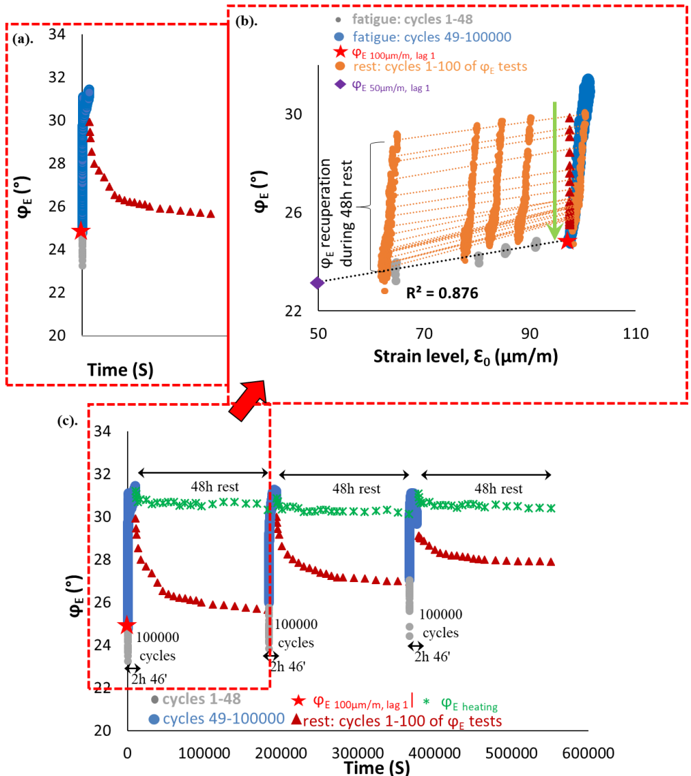
3.1.25. PFRT results obtained for mix 70/100 – 5: (a) \varphi_E as a function of time during the first fatigue lag and rest period (b) \varphi_E as a function of applied strain amplitude during the first fatigue lags and the short complex modulus tests performed within its following rest periods; (c) \varphi_E as a function of time during the three fatigue lags and rest periods (Red stars indicate values of \varphi_E estimated at 100 \mu\text{m}/\text{m} at the beginning of fatigue lag, green asterisk shows values of \Delta\varphi_E heating as influence of self-heating and brown triangles indicate values of \varphi_E estimated at 100 \mu\text{m}/\text{m} for each short complex modulus test during rest (all these values were obtained using non-linearity envelopes, as shown in (b) for the first fatigue lag and rest period).
