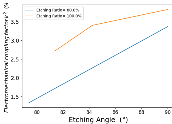
Figure 171: Evolution of k^2 for the TE 2,1 mode with sidewall angle at different etching ratios (Mo/AlN/Mo/SiO 2 /Si, h_{\text{AlN}}/p=1 , a/p=0.5 , h_{\text{bottom}}/p=0.1 , h_{\text{top}}/p=0.1 , h_{\text{SiO}_2}/p=0.5 )
