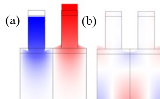
Figure 199: Representation of the mode shape of the pseudo-SAW mode at the entrance ( f = 1.18 GHz) (a) and at the exit ( f = 2.52 GHz) (b) of its stop-band.
