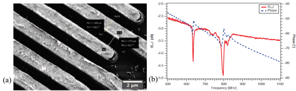
Figure 38: SEM image of the patterned AlScN film by ICP etching, grown on Sapphire (a) Electrical response of a SAW/BAW device of AlScN on Sapphire (b) [81]
