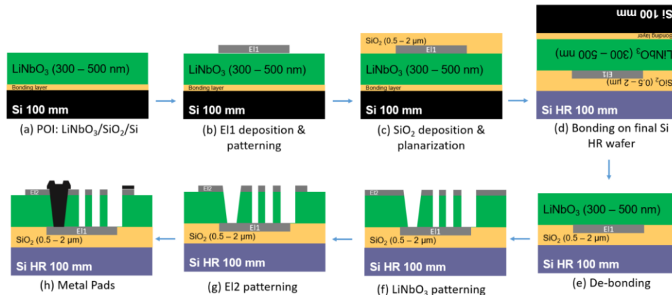
Figure 158: Simplified scheme of process flow for LiNbO 3 HBSR fabrication
