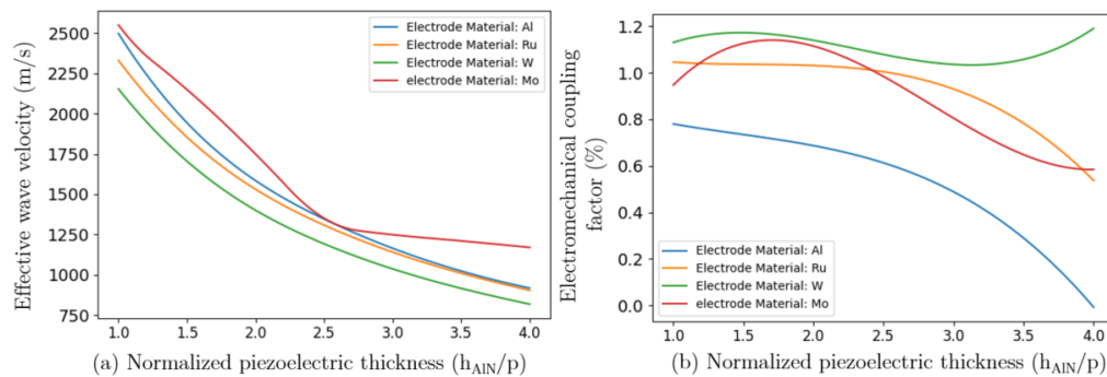
Figure 63: The evolution of the effective wave velocity (a) and k^2 (b) for pseudo-SAW with the transducer thickness for different electrode materials (Metal/AlN/Metal/Si with h/p=2 , a/p=0.5 , El/p=0.16 etching ratio=1 with straight sidewalls).
