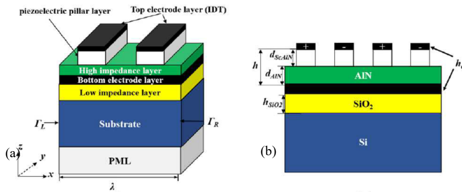
Figure 188: schematic view of the coupled SAW/BAW resonator proposed by Liu et al. in 3D (a) and cross section material and electrical details (b) [86].
