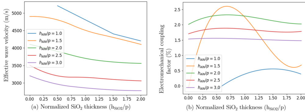
Figure 71: Evolution of the effective wave velocity (a) k_2 (b) for the pseudo-BAW mode with the thickness of the \text{SiO}_2 layer, at different thickness to pitch ratios (Mo/AlN/Mo/ \text{SiO}_2 /Si with a/p=0.5 , El/p=0.16 , with etching ratio=1 and straight sidewalls).
