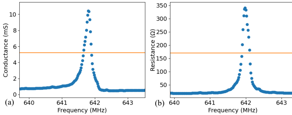
Figure 122: Example of pseudo-SAW resonance (a) and antiresonance (b) with respective quality factors Q_s = 2,900 \pm 450 and Q_p = 3,200 \pm 500 .
