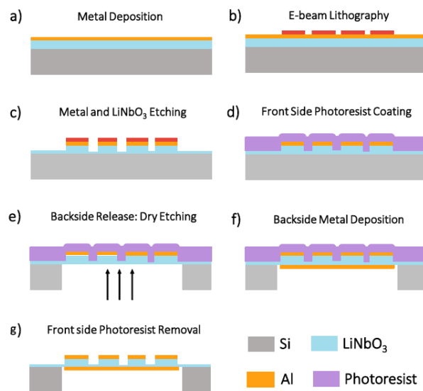
Figure 191: Process flow for YBAR [67] (a) Cr/Al evaporation (b) E-beam lithography with ZEP 520A (c) Ion beam etching of the metal and LiNbO 3 (partially) (d) Photoresist coating as a surface protection layer (e) Silicon DRIE (f) Cr/Al evaporation for bottom electrode (g) Removal of front side photoresist layer by remover 1165.
