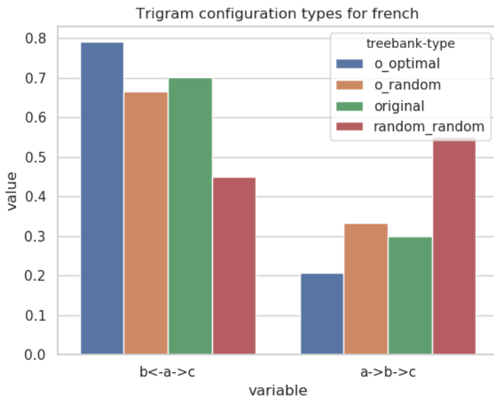
Figure 6.8: Non-linearized trigram configurations distribution for French
