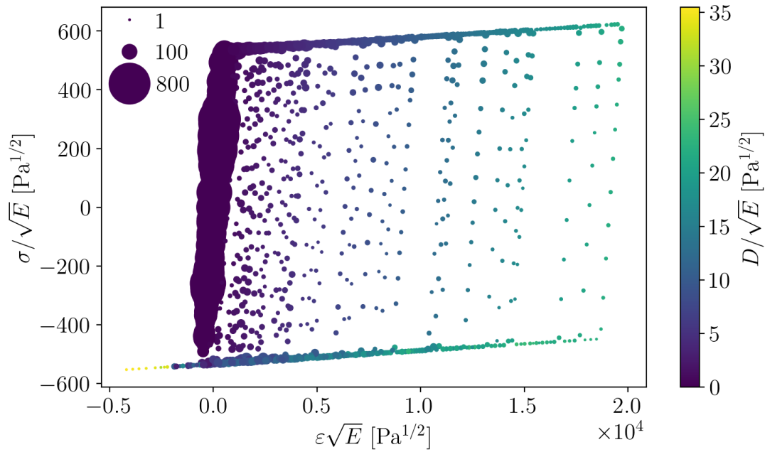
Figure IX.2: Position of clusters in space (\varepsilon\sqrt{E}, \sigma/\sqrt{E}, D/\sqrt{E}) for sampling rate r = 2\% , with marker size symbolising the number of points in a cluster
