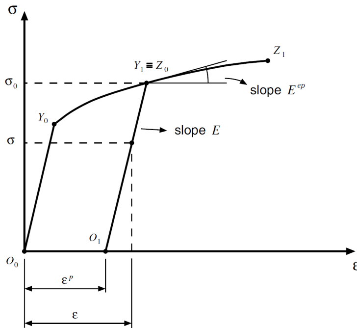
Figure II.1: Uniaxial tension experiment. Mathematical model. From De Souza Neto et al. (2008 [21])
