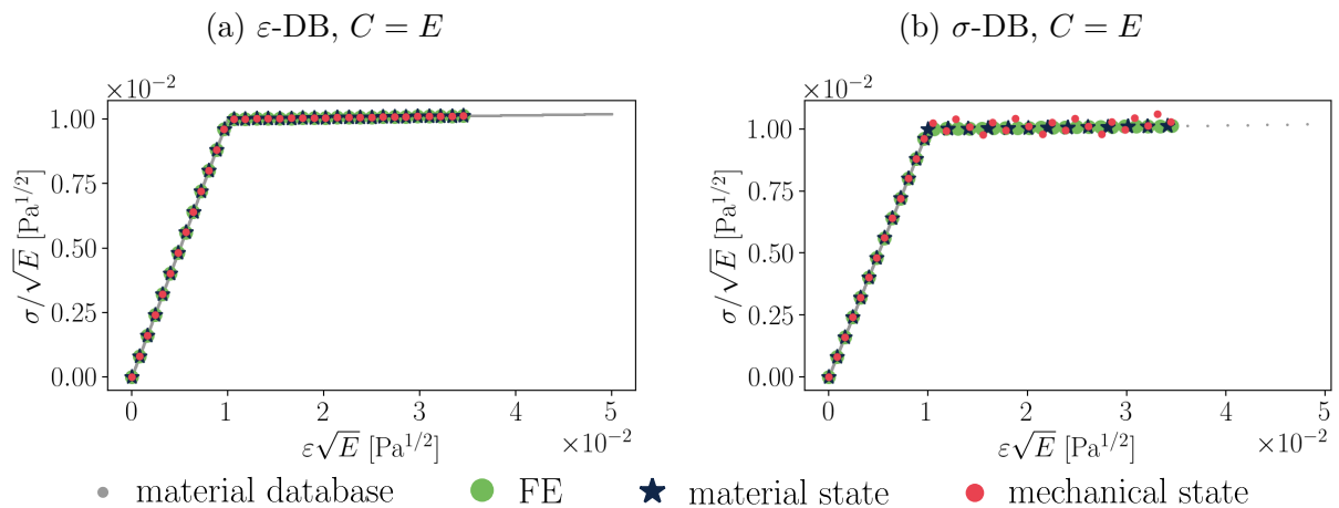
Figure VII.3: Mechanical and material solutions obtained for the elastic spring-bar problem
