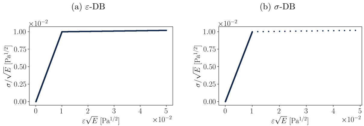
Figure VII.2: Material data sets for the elastic resolution of the spring-bar problem
