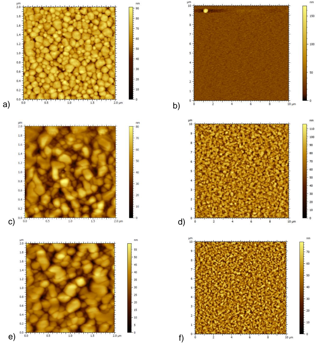
Figure 45. AFM scans for films deposited at RT a) 2 \times 2 \mu\text{m}^2 b) 10 \times 10 \mu\text{m}^2 areas, at 400^\circ\text{C} c) 2 \times 2 \mu\text{m}^2 d) 10 \times 10 \mu\text{m}^2 areas and at 500^\circ\text{C} e) 2 \times 2 \mu\text{m}^2 f) 10 \times 10 \mu\text{m}^2 areas.
