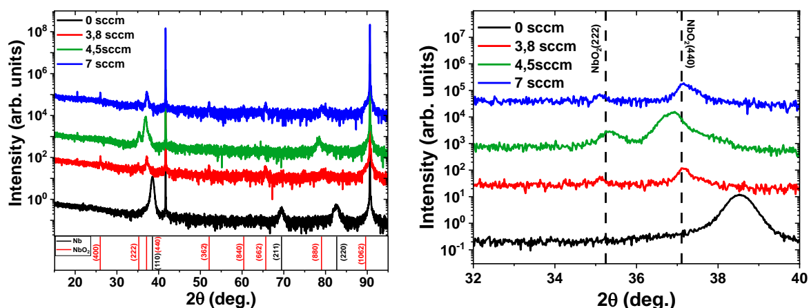
Figure 88. XRD \theta - 2\theta scans of NbO 2 films deposited at different oxygen flows between a) 15° and 95° and b) 32° and 40°.
