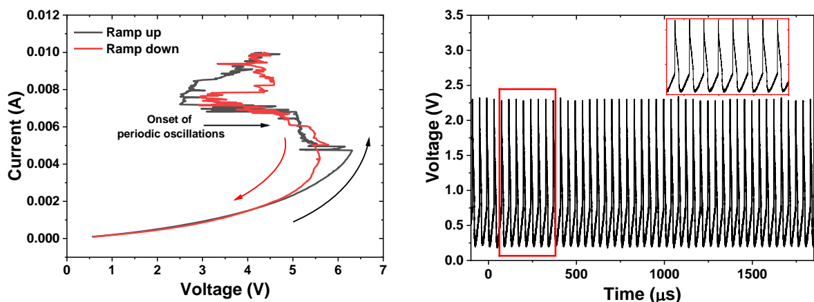
Figure 99. a) I-V characteristic and b) periodic induced voltage oscillations across a NbO 2 – MIM device with an electrode size of 30 \mu\text{m} when excited in the NDR zone with a constant current of 6 mA.
