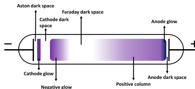
Figure 18. DC glow discharge regions in a typical diode sputtering system.
