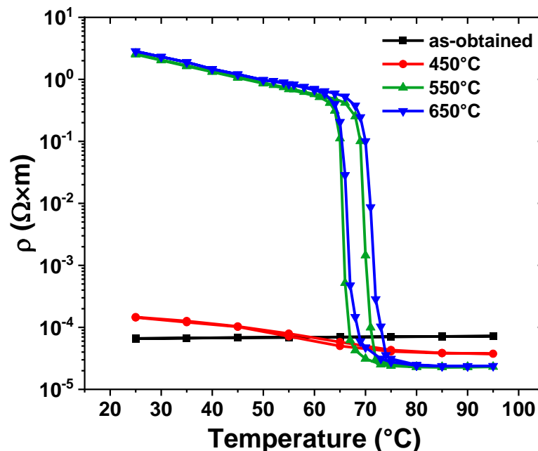
Figure 46. Electrical hysteresis of as obtained and annealed at 450, 550 and 650°C VO 2 films in O 2 atmosphere at 20 mTorr.
