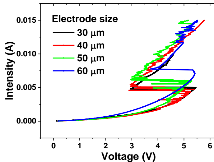
Figure 97. \text{NbO}_2 -based MIM current-based electrical activation for different electrode side sizes.
