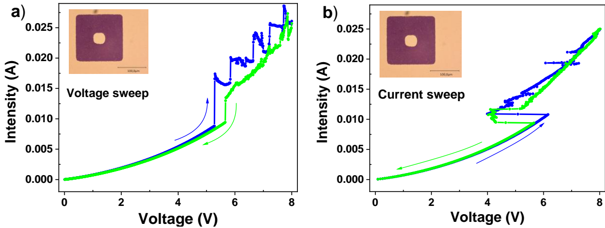
Figure 95. Current-voltage curves subsequent to a) voltage and b) current sweeps applied to the NbO 2 MIM device with an electrode side dimension of 40 μm.
