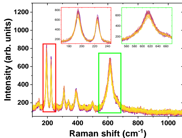
Figure 79. Raman shift evolution at different positions along sample D3 (1.86 at% W) at 100 mA.
