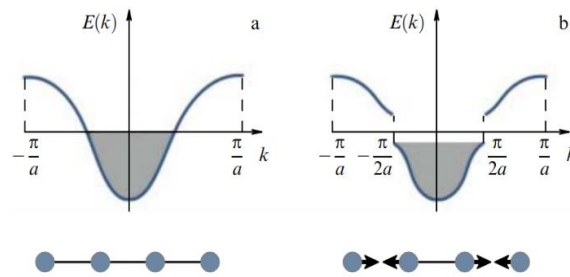
Figure 7. A Peierls transition from an a) undistorted to a b) distorted atom chain, with a bandgap opening at \pm k . [27]
