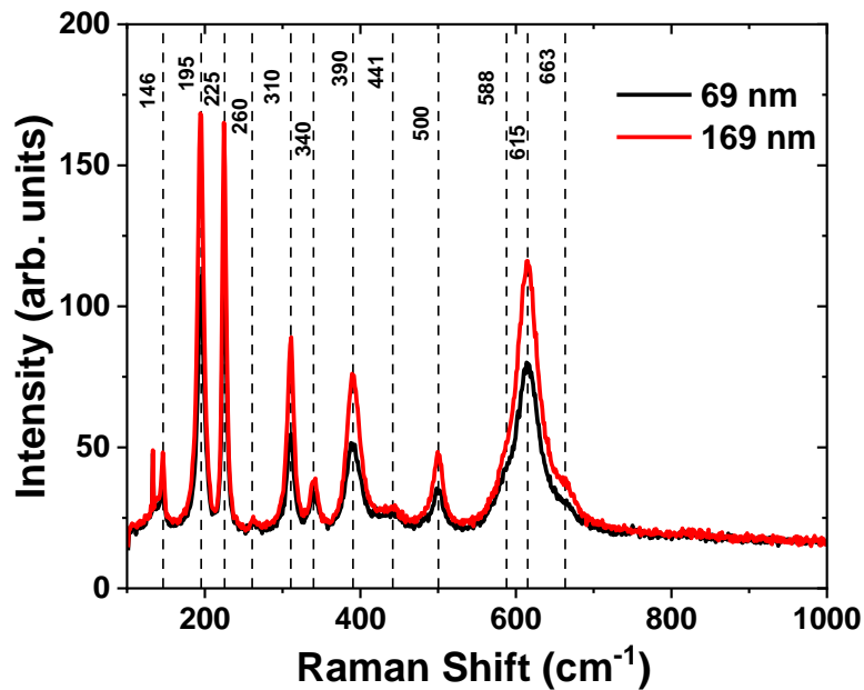
Figure 42. Raman spectroscopy results for VO 2 films of different thicknesses.
