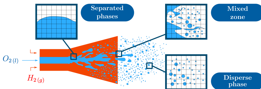
Figure 0.3: Schematic representation of an atomization of cryogenic injectors in aerospace engines (Cordes, 2020).
