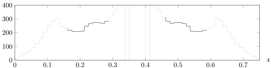
Figure 5.3.6: Profile of \sigma H(\nabla\alpha_1) in Pa. The profile is dashed when the phases are almost pure \alpha_1 > 0.99 and when \alpha < 0.01 .
