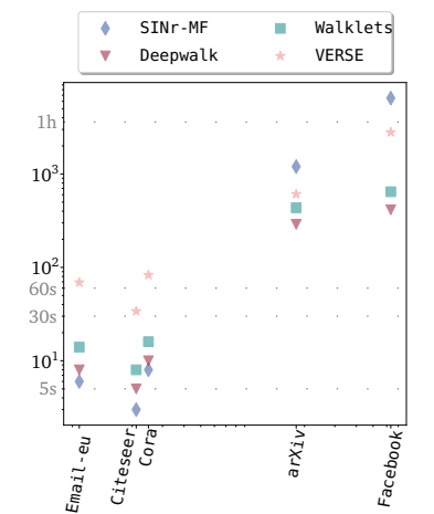
FIGURE 3.5: Slowest methods with regard to the number of nodes.
