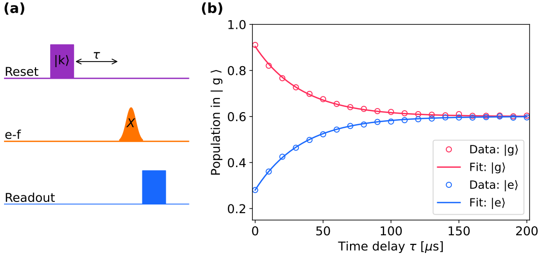
Fig. 6.5 T1 g-e : Measurement of the relaxation time of the |g\rangle \rightarrow |e\rangle transition. (a) Pulse sequence used for the experimental realization: The qubit is initially prepared in either |g\rangle or |e\rangle with the aid of the reset pulse, and then, after waiting a time \tau , the qubit state is determined by the projective measurement consisting of a \pi -pulse ( X ) at the |e\rangle \rightarrow |f\rangle transition and the readout pulse to probe the resonator. (b) Population in the state |e\rangle at the end of each realization as function of the waiting time \tau after the qubit preparation. The empty circles represent the measured data while the solid lines are obtained by fitting the data with an exponential decay. The blue and red colors correspond to a qubit preparation in state |g\rangle or |e\rangle , respectively. The fitted T_1 of the |g\rangle \rightarrow |e\rangle transition is 34\ \mu\text{s} .
