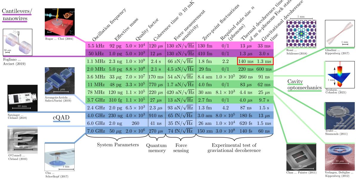
Fig. 0.2 Comparison between various mechanical systems for quantum memory, sensing, and quantum gravity applications. The force sensitivity is calculated using the formula F_{\min} = \sqrt{\hbar m \Omega_m^2 (2n_{\text{th}} + 1)/Q} (see ref. [70]). The state size required for quantum gravity experiments is n = (2.7 \text{ fm}/x_{\text{zpf}})^2 . The corresponding thermal, and gravitational decoherence times are extracted from (0.2) and (0.1) respectively. For mechanical systems where small cat states n < 1 , or even the ground state are sufficient to observe quantum gravitational effects, we write n = 0/1 and calculate the decoherence time in state |1\rangle . The performances of the system envisioned in this proposal are framed in red (see text for details). Images and system parameters are extracted from the following references: Rugar et al. [66], Fogliano et al. [32], Rossi et al. [65], Ghadimi et al. [37], Neuhaus et al. [56], Teufel et al. [73], Verhagen et al. [75], Chan et al. [20], Arrangoiz et al. [6], Satzinger et al. [67], O’Connell et al. [59], Chu et al. [22]. Figure adapted from ref. [35].
