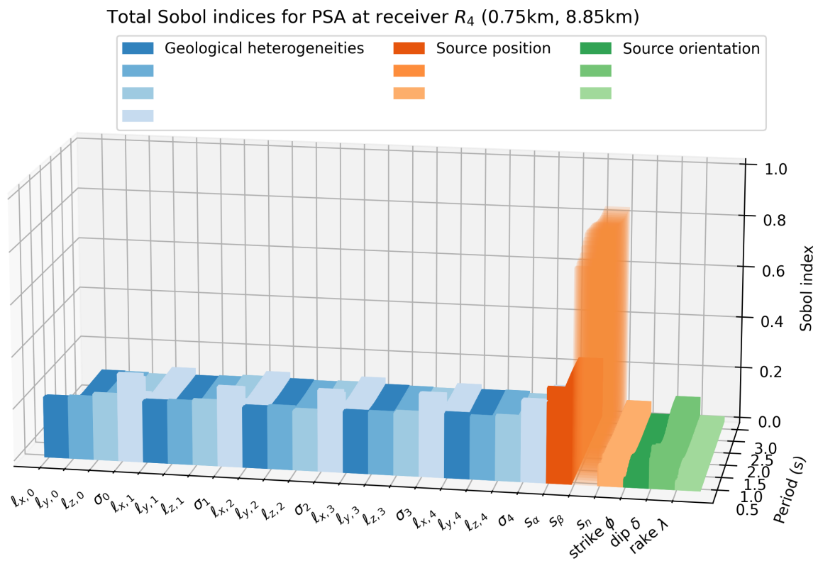
Figure A.31: Total Sobol indices for the PSA on the East-West component computed at receiver R_2 (top) and R_4 (bottom). Each of the 26 parameters is reported on the x axis and the y axis denotes the period.
