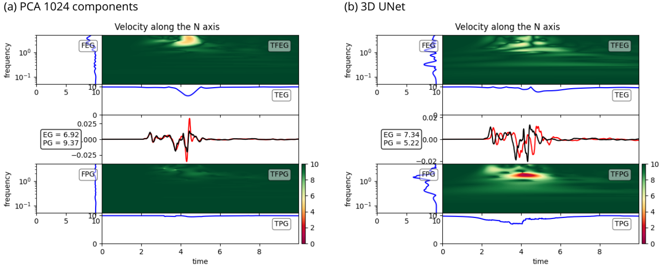
Figure 2.12: For the sensor depicted by the black triangles in Figure 2.11, velocity ground motion along the North-South component. Black: ground motion obtained with the input \bar{V}_S field. Red: ground motion obtained with the \bar{V}_S field reconstructed by (a) PCA and (b) 3D UNet. GOFs are represented in the frequency (FEG and FPG), time-frequency (TFEG and TFPG), and time (TEG and TPG) domain for the envelope (top) and phase (bottom).
