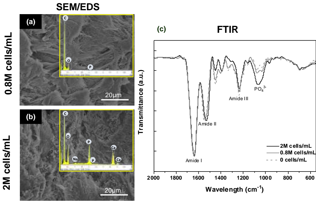
Figure II.9: (a,b) SEM imaging and EDX analysis after 25 days of culture, (c) FTIR spectra of hydrogels after 25 days in culture conditions in the absence of cells and for 0.8 \text{ M.mL}^{-1} or 2 \text{ M.mL}^{-1} initial cell density
