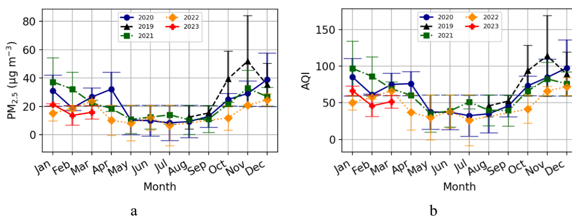
Figure 6.32. Monthly variations of (a) PM 2.5 concentration and (b) Air Quality Index (AQI) for Kyiv during 2019–2023. Measurements by AirVisual, monthly averaged. Years of observation are indicated by colors.
