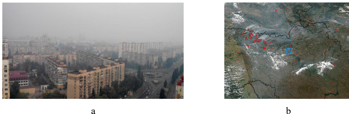
Figure 4.3. a) Haze in Kyiv on September 3, 2015, and b) MODIS satellite image: red dots indicate fires, and the blue circle indicates Kyiv.
