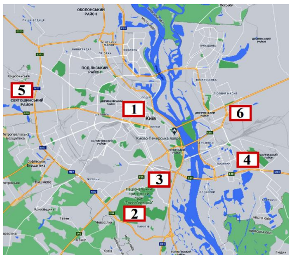
Figure 3.3. Locations of the five AirVisual stations and the Popudrenka station (APDA-371 HORIBA) on the map of Kyiv: 1 – Artema Street, 2 – Golosiiv, 3 – Nauky Avenue, 4 – Trostyanetska, 5 – Chornobylska Street, 6 – Popudrenka.
