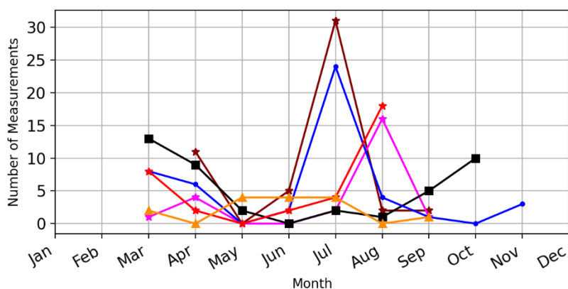
Figure 1. a) Changes of the real part of the complex refractive index at wavelength 440 nm with standard deviation, b) the imaginary part of the complex refractive index at wavelengths 440 nm with standard deviation and c) number of used measurements, 2016, 2017, 2019–2023. Data monthly averaged. Observations from the AERONET station in Kyiv. Years of observation are indicated by colors. Data level 1.5.
