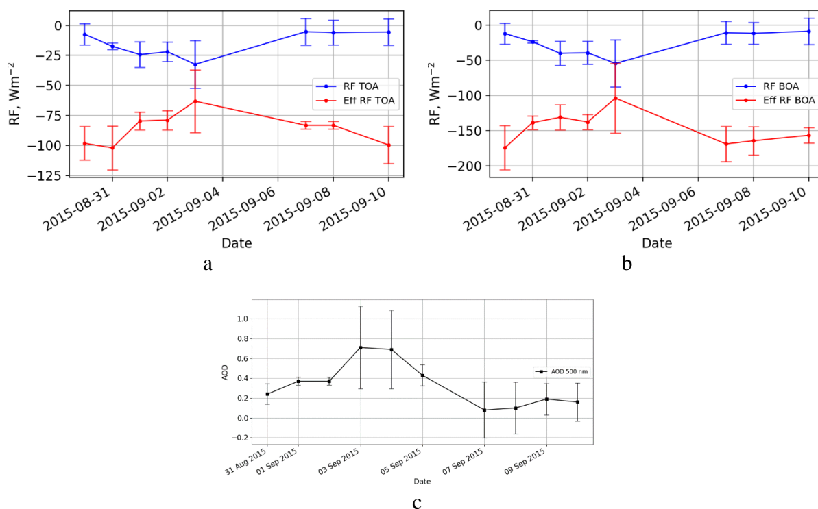
Figure 4.19. Radiative Forcing (RF) and Efficiency of Radiative Forcing (Eff RF) at a) the top of the atmosphere (TOA) and b) the bottom of the atmosphere (BOA); c) AOD (500 nm). Daily average data for the period from August 30 to September 10, 2015, from the AERONET station in Kyiv. AERONET data level 2.0.
