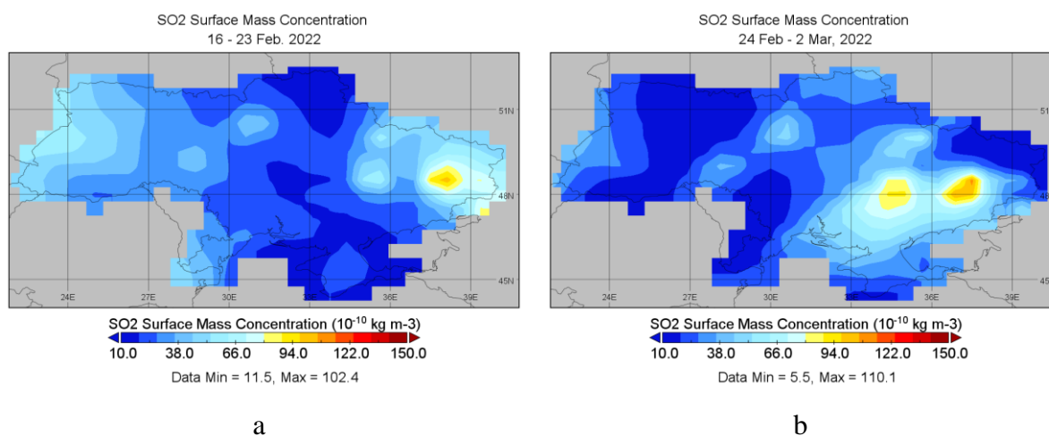
Figure 6.16. Time-averaged surface mass concentrations of \text{SO}_2 in the atmosphere over Ukraine time-averaged for the periods: a) February 16–23, 2022, and b) February 24 – March 2, 2022. Modeling was provided using the MERRA-2 program. Data were obtained from the GIOVANNI platform. The unit of the color scale is 10^{-10} \text{ kg m}^{-3} .
