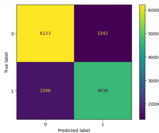
Figure 4.1: Confusion matrix for EXTERNALITY model. There are four values: True Positive (TP) and True Negative (TN) on the diagonal, and False Positive (FP) and False Negative (FN) on the anti-diagonal.
