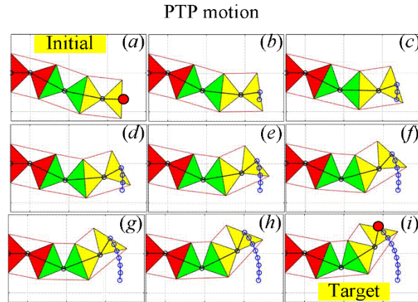
Fig. 4. 16: Kinematic control of the 3-segment manipulator using linear interpolation in (q_1, q_2, q_3) -space and global minimization of the joint increments (PTP motion, objective #b).
