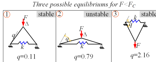
Fig. 1. 20: Mechanism shapes in equilibrium configurations for the loading F_C = 0.5kL , which is lower than F_C = 0.9kL (case \alpha = \pi/3 ).
