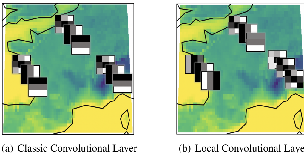
Figure 24 – Left: standard CNN with same convolutional kernel layers convolved along the entire image. Right: localized convolution layer with different kernels in each part of the image.
