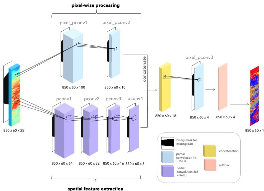
Figure 51 – Chosen architecture for the Partial Convolutional Neural Network.
