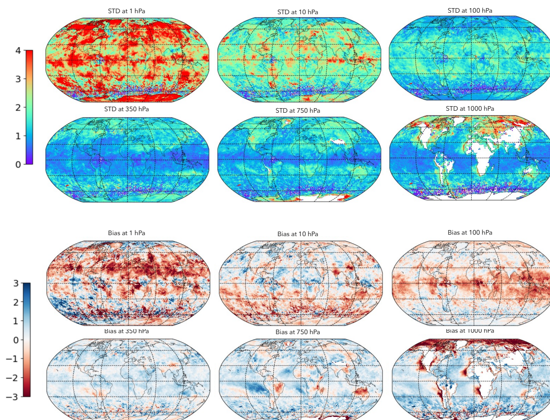
Figure 67 – Average STD (top) and Bias (bottom) errors between the retrieval and ERA5 temperatures at 1, 10, 100, 350, 750 and 1000 hPa in kelvins on a 1^\circ grid. Fewer pixels are plotted in the lower layers due to changes in surface pressure.
