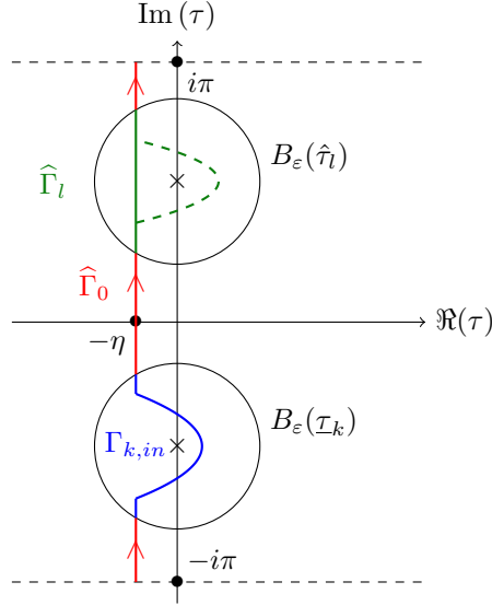
Figure 2.4 – This is a representation of \Gamma_k where we decompose \Gamma_{k,out} . The red path corresponds to \hat{\Gamma}_0 the part of \Gamma_{k,out} which lies outside the balls B_\epsilon(\hat{\tau}_l) . The green path corresponds to \hat{\Gamma}_l the part of \Gamma_{k,out} which lies inside the ball B_\epsilon(\hat{\tau}_l) . The dashed green path corresponds to the deformation we use in the proof of the estimate for E_1 .
