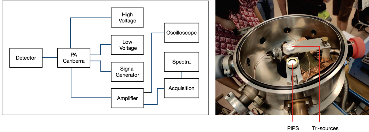
Figure 62: Diagram showing the setup used for testing the 13 potentially usable PIPS detectors for the experiment. The photo on the right displays the interior of the reaction chamber before the vacuum is applied, with the detector positioned approximately 13 cm away from the source in a vertical plane.
