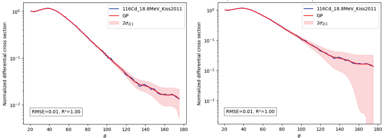
Figure 70: Plots illustrating the angular cross section of the ^{116}\text{Cd}(\alpha, \alpha) reaction at 18.8 MeV. The blue points represent the experimental data, while the red curve corresponds to the GP fits. In both studies, the same kernel has been used, which include white noise. On the right plot however, the allowed range of the white noise parameter has been set to a lower limit. The pale red shading around the fit represents the deviation from the mean, captured by the standard deviation. This subtle variation in the plots arises from minor adjustment in the kernel parameterization.
