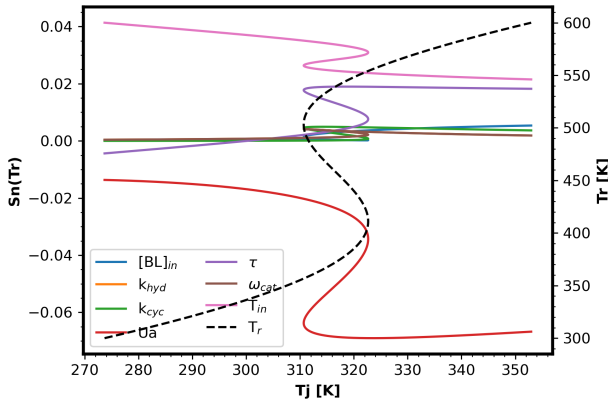
(e) Tr PSA for Ua=800 \text{ W/m}^3/\text{K} .
