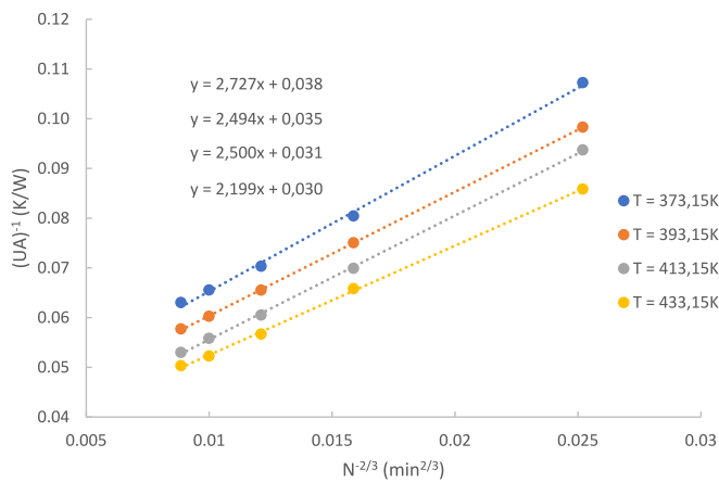
Fig. 3. Wilson plot.
