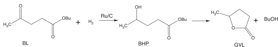
Fig. 2. Reaction pathway for the hydrogenation of BL over Ru/C.
