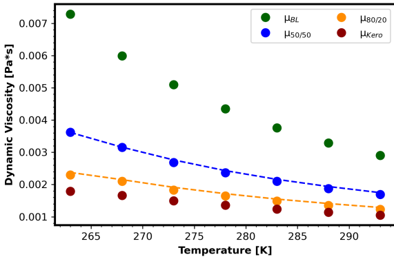
(c) Dynamic Viscosity vs Temperature.
