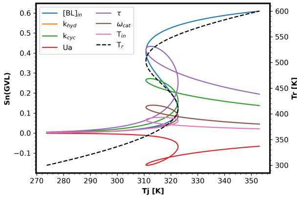
(c) GVL PSA for Ua=800 \text{ W/m}^3/\text{K} .
