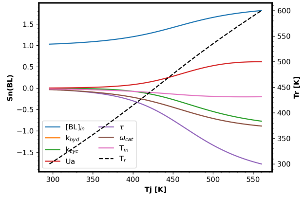
(b) BL PSA for Ua=5000 \text{ W/m}^3/\text{K} .
