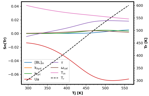
(f) Tr PSA for Ua=5000 \text{ W/m}^3/\text{K} .
