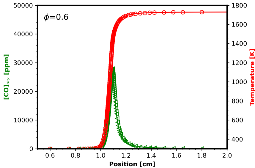
(a) 1D n-heptane computational flame for \phi=0.6 .
