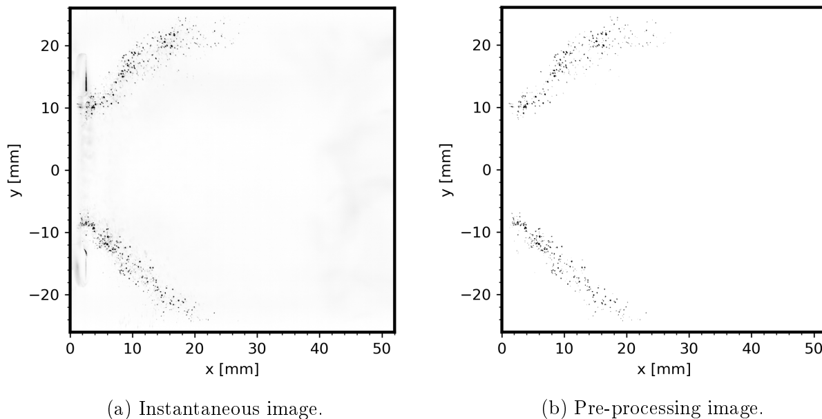
Figure 5.24 Spray instantaneous image of pure kerosene at OP_1 and \phi=0.51 .
