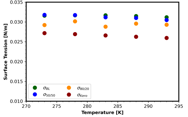
(b) Surface Tension vs Temperature.
