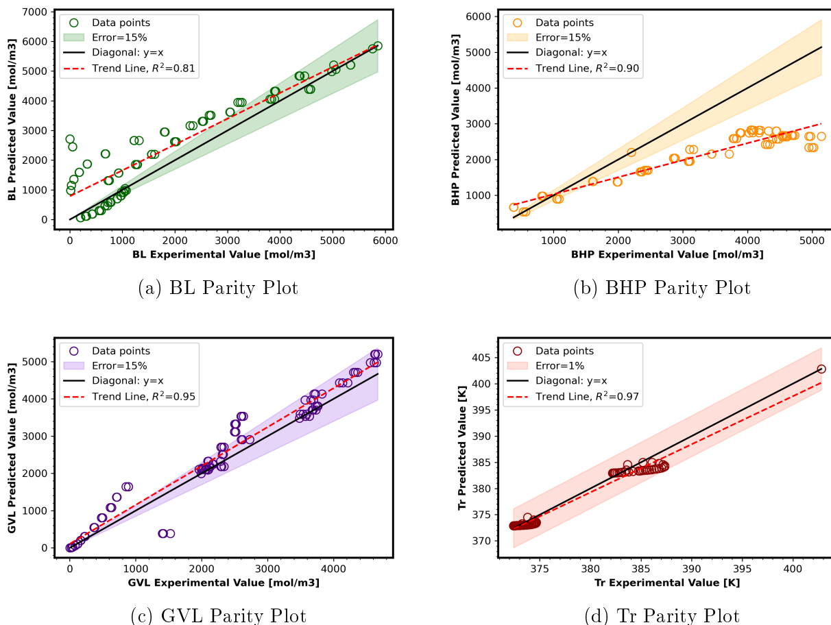
Figure 3.14 Validation Stage Parity Plot, NCLH1 kinetic model.
