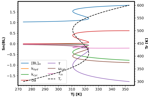
(a) BL PSA for Ua=800 \text{ W/m}^3/\text{K} .
