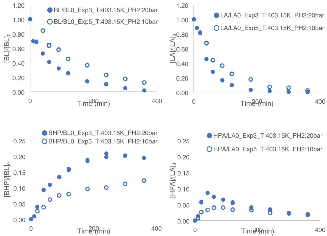
Fig. 5. Effect of pressure on the kinetics of hydrogenation and cyclization steps for experiments 3&5.
