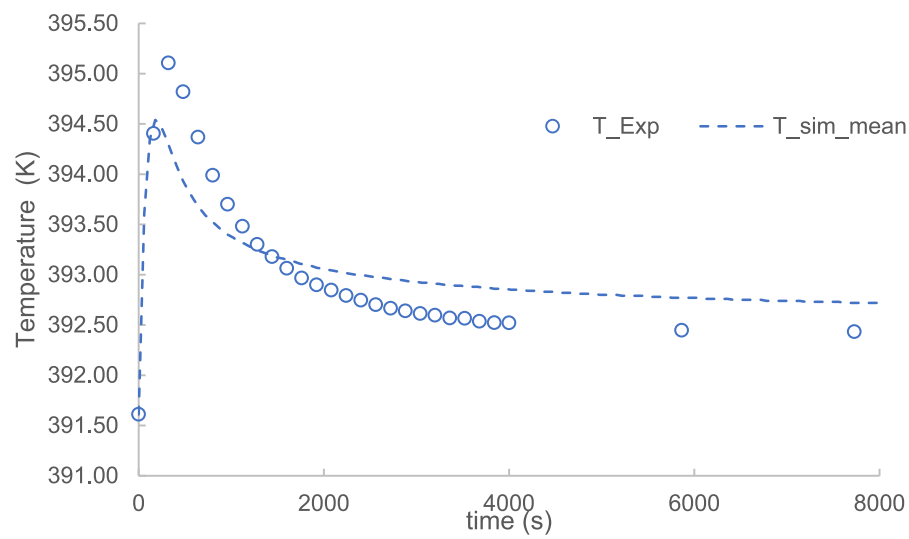
Fig. 5. Fit of the NCLH1 model to isoperibolic experimental data for Run 2.
