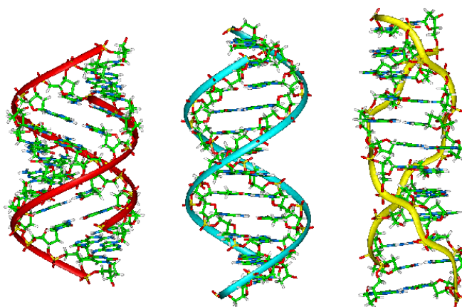
Figure 1.4: Three possible DNA double-helix structures. From left to right, A , B and Z forms. The ribbons represents the phosphate-sugar backbone.
