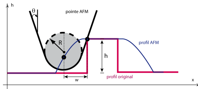
(b) Convolution between the sample and the probe for AFM measurements (figure from [Mon08]). The dilation effect depends on the size of the tip R , and the height of the object h .
