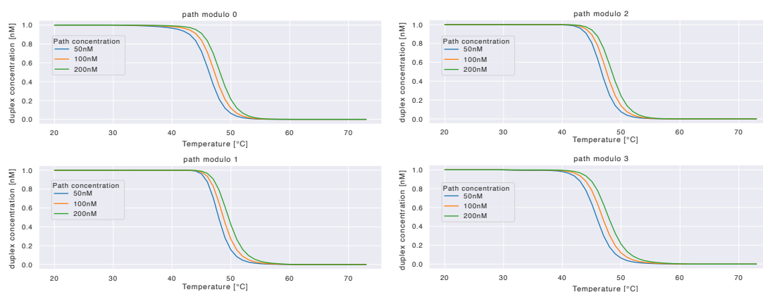
Figure 5.16: Melting curves of pairs of weaker binding path strands. The signals are processed to show the melting curve as if there were 1 nM of one strand (simulating 1 nM of origami), and 50 nM to 200 nM of the other strand.
