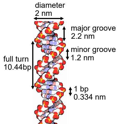
Figure 1.6: Space filling representation of a DNA double helix, with size annotations.
