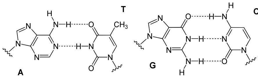
Figure 1.2: Possible hydrogen bonds between the bases Adenine - Thymine and Guanine - Cytosine . The dashed lines represent the connections to the sugars of the nucleotides. The pair G-C can form one more hydrogen bond, which enhances its stability.
