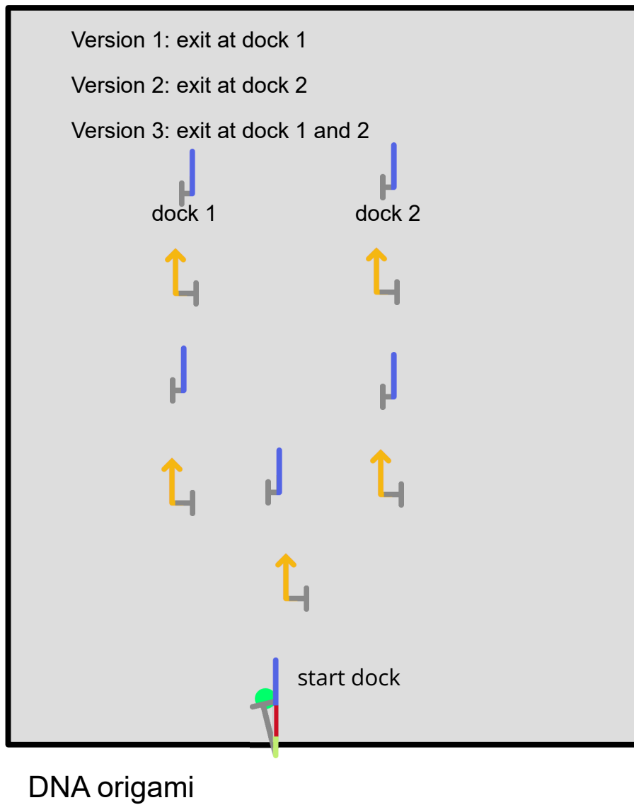
Figure 6.11: Branching experiment
