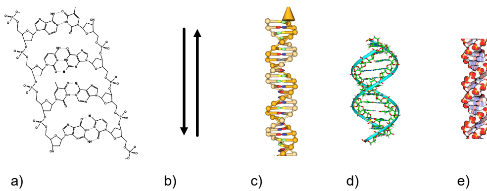
Figure 1.3: Representations of double-stranded DNA. a) Chemical structure of a double strand with four nucleotides. b) Schematic representation of complementary domains. Each line represents a DNA strands. The arrow indicates the 5' to 3' direction. c) DNA ball-and-stick representation. A pair of adjacent ball and stick represents a nucleotide. The inner colored oval ball at the end of a stick represents a base. d) Chemical ball-and-stick representation. The added ribbons represents the sugar-phosphate backbone which are alligned on the phosphate atoms. e) Space filling representation.
