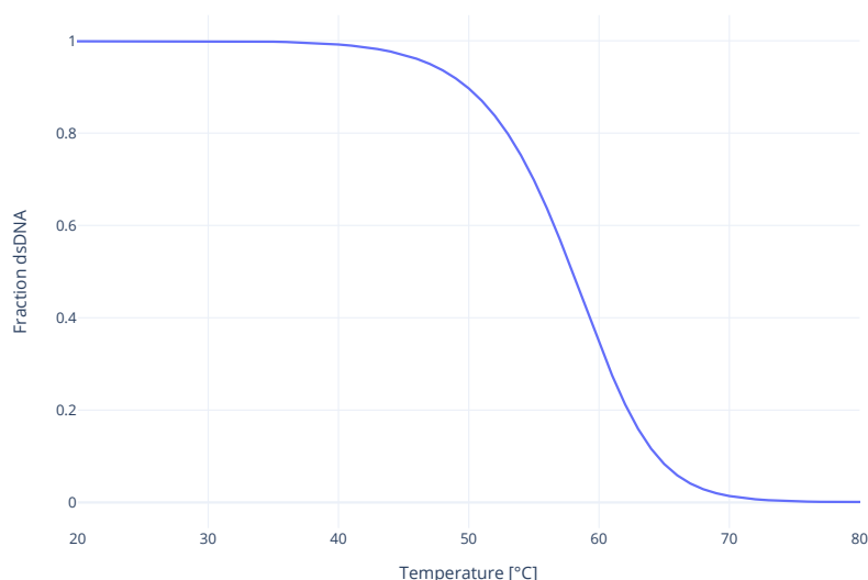
Figure 1.8: Fraction of dsDNA at equilibrium in function of the temperature. Prediction was made with Nupack software with 1 \mu\text{M} of strand with sequence ATGCAGGATCAGTATA and 1 \mu\text{M} of its complementary strand, in 12.5 mM Magnesium.
