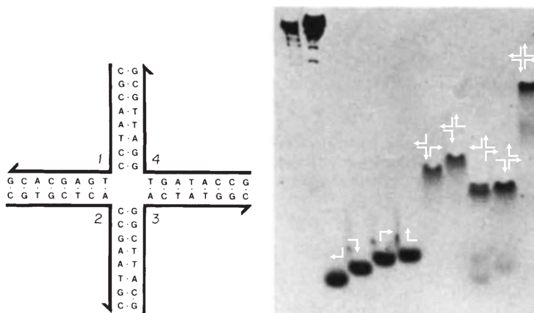
(a) Sequences for the immobile four-way junction. (b) Acrylamide gel of the self assembled four-way junction structure.
