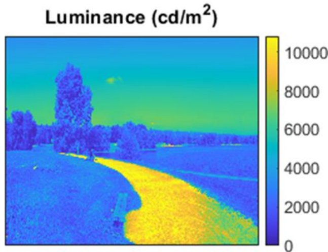
Figure 56, Sample Luminance map for an outdoor scene
