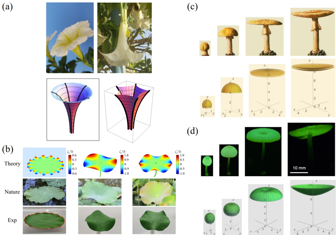
Figure 1.9 – (a) Above: A surfinia (Paris) and An Angel's trumpet (brugmansia) (Morocco). Below: their simulation images [111]. (b) Morphological comparison of different types of lotus leaves. Left: A floating lotus leaf grows with short waves along the edge (the wavy edge is highlighted by red color in experiments). Medium and right: suspended lotus leaves morph into long-wavelength ripples [112]. (c) Above: The cap morphological development of the mushroom Amanita muscaria . Below: Simulation images of different parameters. (d) Above: The cap morphological development of the mushroom Mycena chlorophos . Below: Simulation images of different parameters [113].
