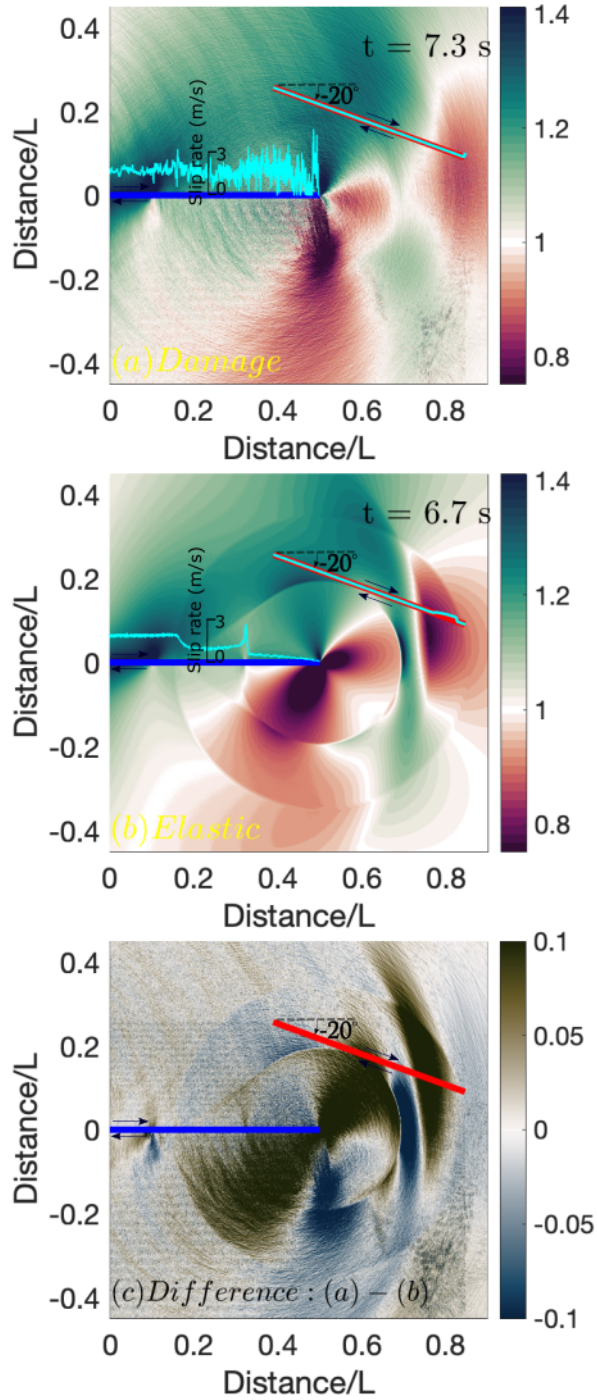
Figure 5.36: Case vii ( \Psi = 67.9^\circ, \omega = -20^\circ ): (c) comparison of normalized normal stress ( \sigma_{yy(\omega)}/\sigma_{yy(\omega)}^o ) for a dynamic rupture on compressional stepover faults embedded in (a) damage and (b) elastic medium. Strike-slip faults are represented by straight lines colored in blue (fault 1) and red (fault 2). Stresses are rotated respect to the orientation \omega of fault 2. Initial orientation of the maximum principal stress \sigma_1 defined by the angle \Psi is measured respect to the strike of the fault 1. White color in figures (a) and (b) labels the initial normal stress. Slip rate on the faults (curves colored in cyan) is superimposed on the snapshots. Length of fault 1, L = 28 km. Parameters are summarized in table 5.1 and 5.2.
