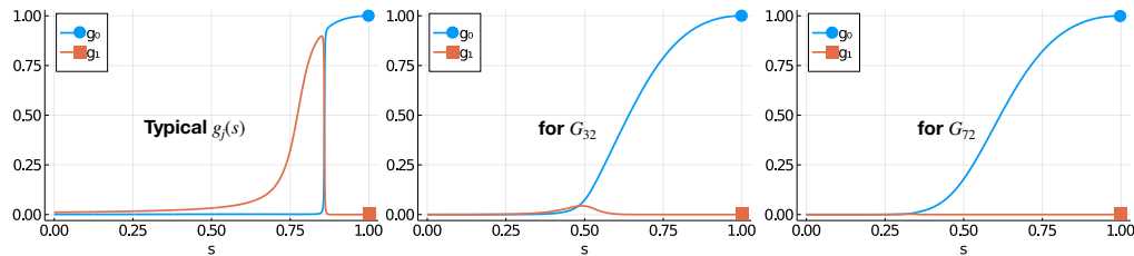
Figure 4.13: Evolution of g_0(s) in blue and g_1(s) in red for graph G_{72} (right), G_{32} (middle) and a typical behavior (left) during an AC like in Section 3.2.
