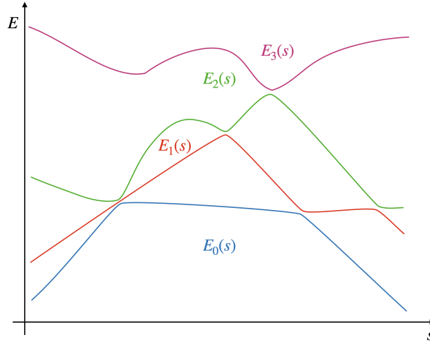
Figure 3.9: Example of an energy spectrum in which the ground-state undergoes two anti-crossing. In this situation, the first AC does not follow our definition but the second one does.
