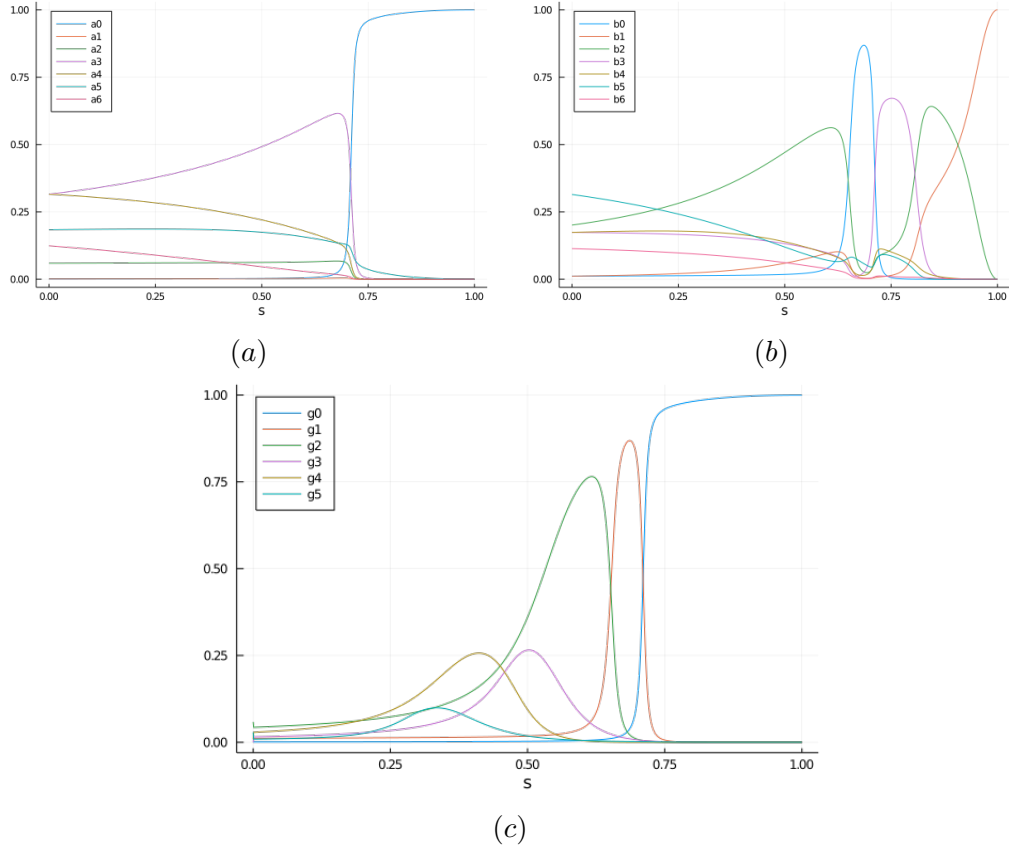
Figure 3.8: a_k (a), b_k (b) and g_k (c) during evolution for toy example 3.6 with \alpha = 0.2 . Values indexed by 0 are in blue, those by 1 in red, 2 in green and 3 in purple.
