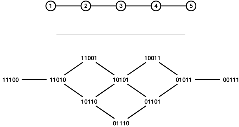
Figure 2.6: Example of a connected G_{\text{driver}} , a line on n = 5 nodes (top) and the generated search graph (down) with adjacency matrix -H_0 associated to the given driver graph where we implicitly fix k = 3 .
